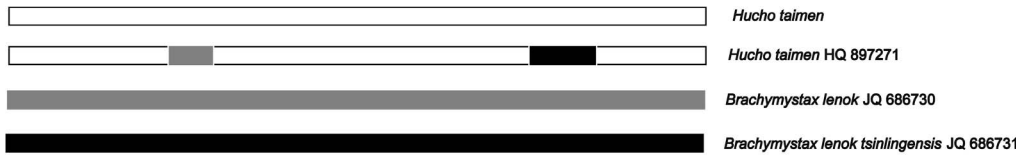
Figure 5. Schematic representation of the recombination events in the mitochondrial DNA of Hucho taimen from the Hutou range (GenBank HQ897271). The top parental sequence is from H. taimen (our study); the two bottom parental sequences are from B. lenok (first recombination event, in grey) and B. lenok tsinlingensis (second recombination event, in black). doi:10.1371/journal.pone.0071147.g005
