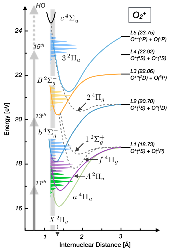
FIG. 2. (color online) Selected potential energy curves of the molecular cation O_2^+ . The harmonics 11 th (16.9 eV), 13 th (20 eV), and 15 th (23 eV) coherently populate several electronic states, as illustrated in the figure as vertical grey arrows. Nuclear-wave-packets are created in several potential energy curves in the Franck-Condon region (indicated by a vertical line at 1.25 Å), from where the molecular ion dissociates into several limits, labeled as L1-L5.
