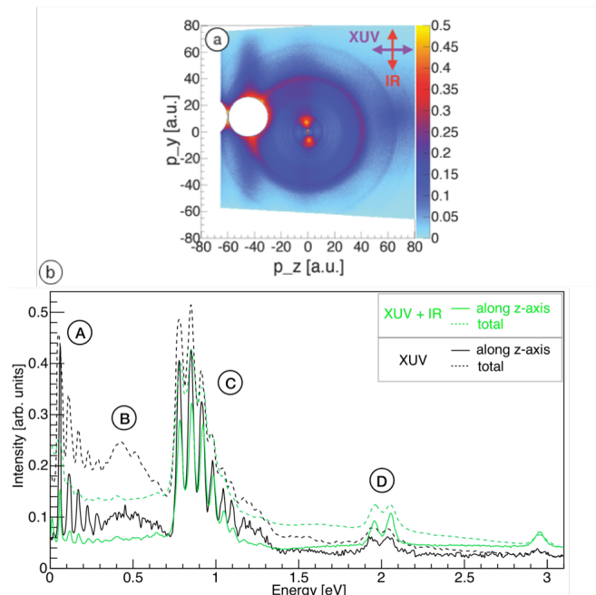
FIG. 4. (color online) a) O^+ 2D ion momenta in the y-z plane after dissociation of O_2 molecules using XUV pulses (16.9 eV, 20 eV, and 23 eV) in the presence of the phase-locked orthogonal IR field in the pump arm. The contributions from stable OH^+ and H_2O^+ ions have been blocked out in this multi pulse scheme only (white circles). b) Kinetic energy of the O^+ ions after dissociation of O_2 molecules. The dark solid and dashed lines show the kinetic energies of the O^+ using XUV pulses only (same as figure 3b). The light solid and dashed lines represent the data with the simultaneous action of the XUV and IR fields. The dashed lines show the result averaged over all fragmentation angles. The solid lines represent the molecular breakup in a cone (with an open angle of 37^\circ ) along the XUV polarization axis (z-axis, i.e. TOF axis). The letters (A, B, C, and D) mark four different features and are used in the discussion. We note that the data here are analyzed in the p_z - p_y plane and should not be directly compared with the data analyzed in the p_z - p_x plane due to the slightly different slicing conditions done in the analysis.
