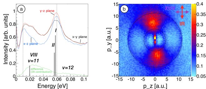
FIG. 5. (color online) (a) O^+ ion energies corresponding to different conical slices (collars with an open angle of 37^\circ ) in the (black) x-y momentum plane, i.e. where the XUV pulse is out of plane, (blue) x-z momentum plane, i.e. where the IR is out of plane, and (red) y-z momentum plane, i.e. where both XUV and IR are in plane. The difference (green) of (y-z plane)-(x-z plane) possibly removes most of the XUV-only contribution. b) detailed view of the O^+ ion momentum distribution in the y-z momentum plane, i.e. where both XUV and IR are in plane.
