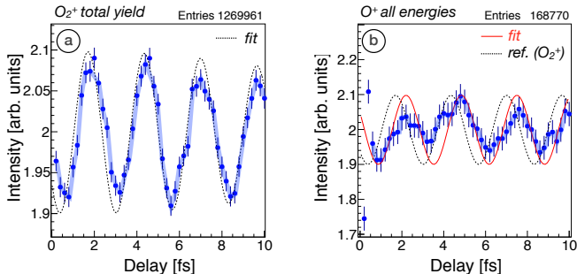
FIG. 7. (color online) Time dependent ion yields with respect to the pump (XUV+IR) - probe (IR) delay. (a) Total \text{O}_2^+ ion yield, (b) total \text{O}^+ ion yield. A cosine fit to the \text{O}_2^+ ion yield is shown as a dashed line in (a) and (b). A cosine fit to the \text{O}^+ ion yield is shown as a solid line.
