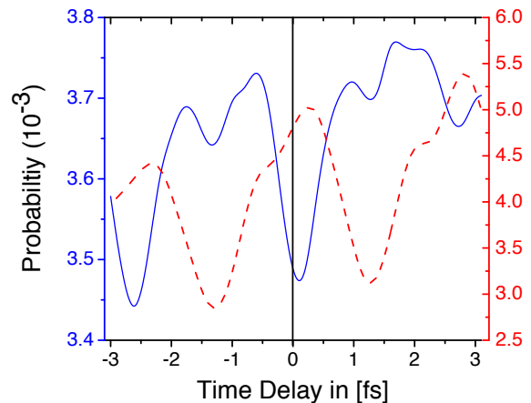
FIG. 9. (color online) Calculations of the time dependent O + ion yields show periodic oscillations for different orientations of the molecular axis as a function of the delay between the XUV and IR pulses. In the calculation, we used the XUV intensity of 3.5x10 10 W/cm 2 . Because of the medium field strengths and the low Z of the oxygen target the spin-orbit approximation is valid, which allowed us to perform a spin-averaged simulation. Dashed line: parallel orientation of the molecular axis and the XUV polarization. Solid line: molecular orientation parallel to the IR polarization. These yields are averaged over all electronic states.
