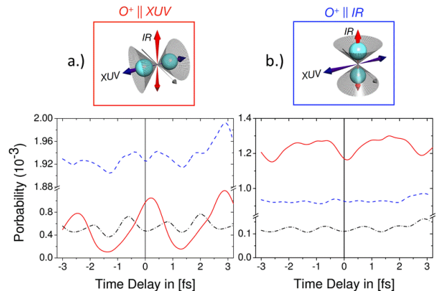
FIG. 10. (color online) State selective calculations of the time dependent O^+ ion yields show a periodic oscillation for different orientations of the molecular axis as a function of the delay between the XUV and IR pulses. (a): parallel orientation of the molecular axis and the XUV polarization. (b): molecular orientation parallel to the IR polarization. Black (dot-dashed) lines: \Sigma states. Blue (dashed) lines: \Pi_g states. Red (full) lines: \Pi_u states.
