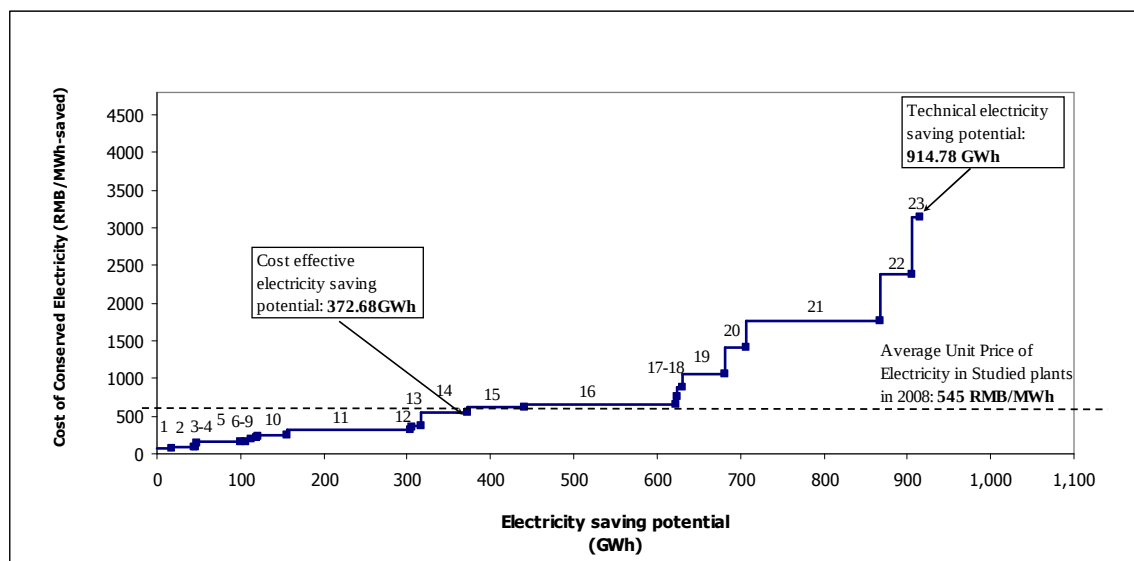
Figure 14. Electricity Conservation Supply Curve (ECSC) for 16 Studied Cement Plants in Shandong Province
