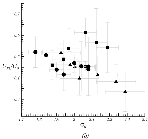
Figure 29: (a) The propagation speed of the void fraction front measured in the laboratory frame, U_{FL} , versus cavitation number, \sigma_0 , for three freestream speeds U_0 = 6 \text{ ms}^{-1} ( \blacktriangle ), 8 \text{ ms}^{-1} ( \blacksquare ), and 10 \text{ ms}^{-1} ( \bullet ); (b) the data plotted as the ratio U_{FL}/U_0 .
