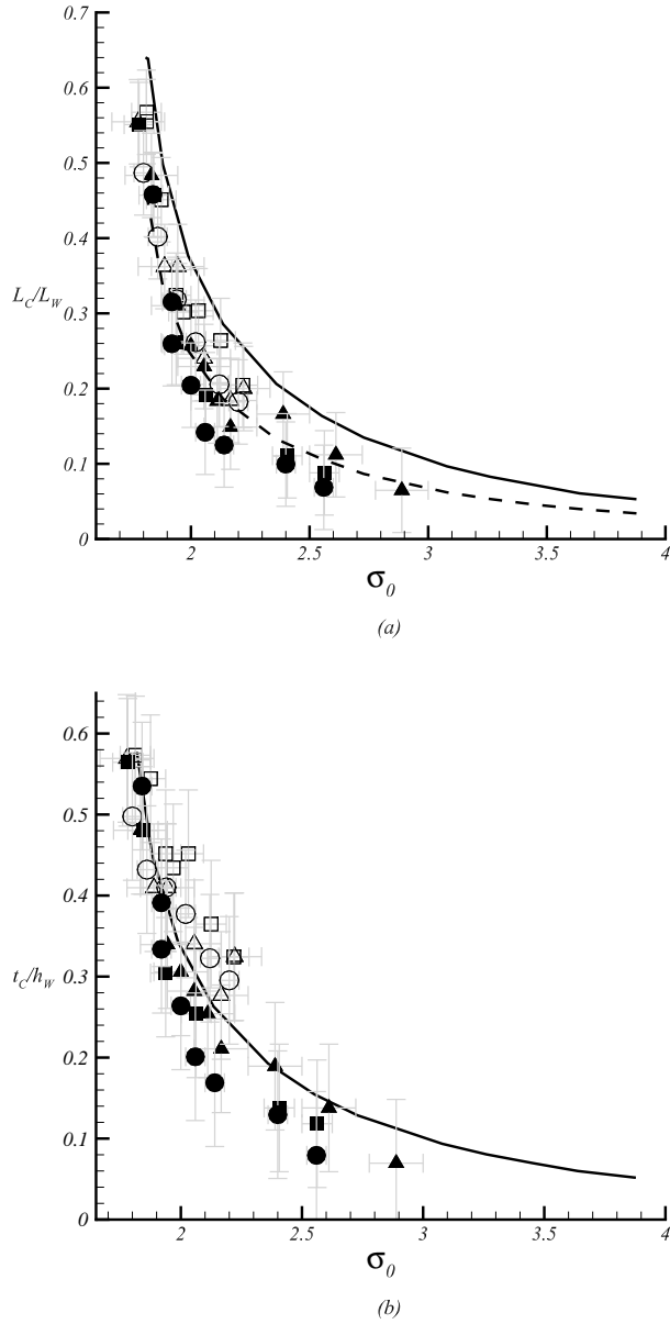
Figure 6: Variation of (a) average cavity length, L_C/L_W , and (b) maximum cavity thickness, t_C/h_W , with cavitation number, \sigma_0 , for three inlet speeds U_0 = 6 \text{ ms}^{-1} (▲), 8 \text{ ms}^{-1} (■), and 10 \text{ ms}^{-1} (●). The open symbols are measurements from the video images, and the filled symbols are from the X-ray images. For periodically shedding cavities ( \sigma_0 < 1.9 ), the maximum cavity length L_{CM}/L_W is plotted. Also shown in (a) are the solution from the free-streamline theory for the cavity length (solid line), and the length to the point of maximum cavity thickness (dashed line); the solution for the maximum cavity thickness is shown in (b).
