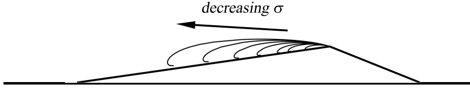
Figure 4: Example solutions for the cavity profile for varying cavitation numbers \sigma = 3.33, 2.80, 2.61, 2.39, 2.24, 2.13 and 2.07 .
