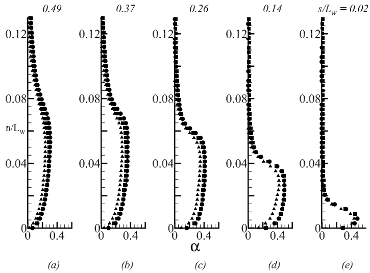
Figure 19: Surface normal profile of \langle \alpha \rangle for the periodically shedding cavity at locations s/L_W = 0.49, 0.37, 0.26, 0.14, \text{ and } 0.02 (a) through (e) for \sigma_0 = 1.95 and three freestream speeds U_0 = 6 \text{ ms}^{-1} ( \blacktriangle ), 8 \text{ ms}^{-1} ( \blacksquare ), and 10 \text{ ms}^{-1} ( \bullet ).
