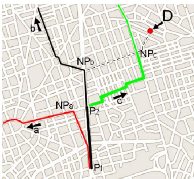
Fig. 2 GeOpps Neighbor Selection, where their routes are evaluated with respect to the potential “Nearest Point” (NPx) to the destination D
