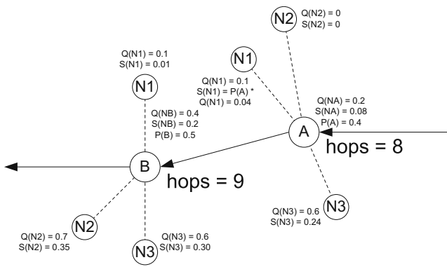
Fig. 10 Routing example 1
