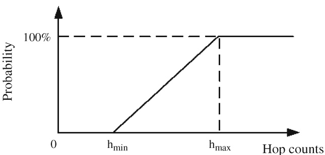
Fig. 8 Function P(h)
