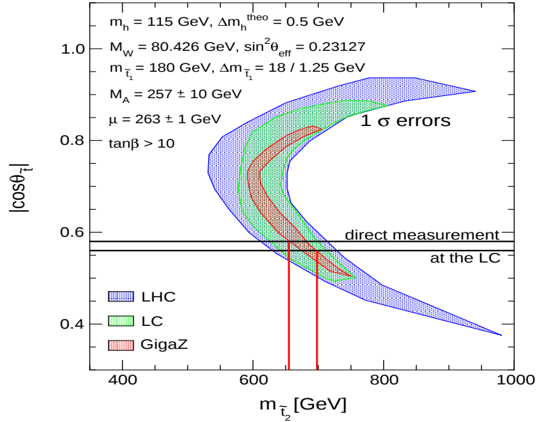
Figure 8.3: Indirect constraints on the MSSM parameter space in the m_{\tilde{t}_2}-|\cos\theta_{\tilde{t}}| plane from measurements of m_h , m_W , \sin^2\theta_w^{\text{eff}} , m_t and m_{\tilde{t}_1} at a LC with and without the Giga-Z option and at the LHC. The solid lines indicate the direct information on the mixing angle from a measurement at the LC and the corresponding indirect determination of m_{\tilde{t}_2} .
