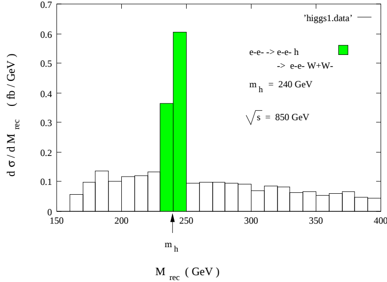
Figure 14.1: Differential cross sections as functions of recoil mass for e^-e^- \rightarrow e^-e^- h and its principal standard model background e^-e^- \rightarrow e^-e^- W^+W^- . The Higgs boson mass is m_h = 240 GeV, \sqrt{s} = 850 GeV, and each electron satisfies an angular cut \theta_{e^-} > 5^\circ . From [7].
