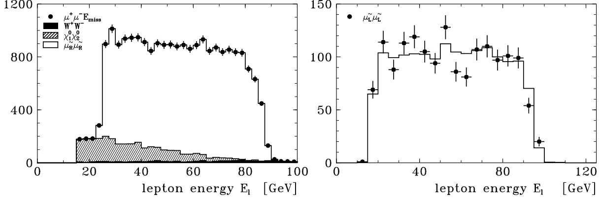
Figure 2.7: Energy distribution of muons resulting from processes e^+e^- \rightarrow \tilde{\mu}^-\tilde{\mu}^+ , followed by \tilde{\mu} decay, from [77]. left: e^+e^- \rightarrow \tilde{\mu}_R^-\tilde{\mu}_R^+ , for a 160 \text{ fb}^{-1} event sample at 320 GeV; right: e^+e^- \rightarrow \tilde{\mu}_L^-\tilde{\mu}_L^+ , with selection of \tilde{\mu}_L \rightarrow \mu\tilde{\chi}_2^0 , \tilde{\chi}_2^0 \rightarrow \ell^+\ell^-\tilde{\chi}_1^0 decays on both sides, for a 250 \text{ fb}^{-1} event sample at 500 GeV. The electron beam polarization is used to reduce the background from e^+e^- \rightarrow W^+W^- .
