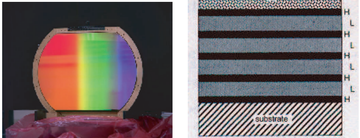
Figure 13.10: The 94 cm aperture gold-coated diffraction grating used for pulse compression on the Petawatt laser is shown on the left. A multilayer dielectric grating design of high-index (H) and low-index (L) layers and groove corrugations (G) is shown on the right. Layers form a high-reflectivity stack under the corrugations.
