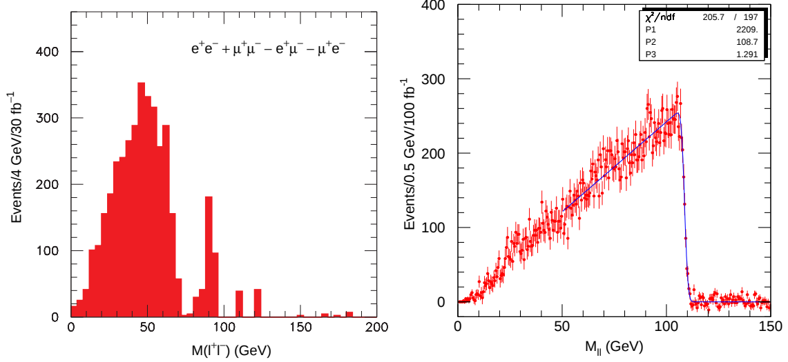
Figure 4.14: Plot of the e^+e^- + \mu^+\mu^- - e^\pm\mu^\mp mass distribution for LHC SUGRA Point 4 with direct \tilde{\chi}_2^0 \rightarrow \tilde{\chi}_1^0 \ell\ell decay (left) and for LHC SUGRA Point 5 with \tilde{\chi}_2^0 \rightarrow \tilde{\ell}^\pm \ell^\mp \rightarrow \tilde{\chi}_1^0 \ell^+ \ell^- (right) [252]. The event generator ISAJET is used. The shape of the peak on the left plot below 70 GeV should be compared to the shape of the peak in the right plot. The left plot also contains a Z \rightarrow \ell^+ \ell^- signal that comes from heavier gauginos.
