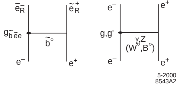
Figure 2.10: Comparison of the weak interaction coupling g' and its supersymmetric counterpart g_{b\tilde{e}e} .
