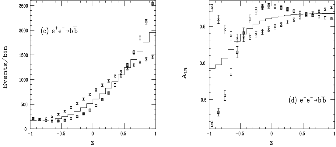
Figure 5.14: Bin-integrated angular distribution and z -dependent ( z = \cos \theta ) left-right asymmetry for e^+e^- \rightarrow b\bar{b} at \sqrt{s} = 500 GeV. The solid histogram represents the Standard Model while the ‘data’ points are for M_* = 1.5 with \lambda = \pm 1 . The error bars indicate the statistics in each bin.
