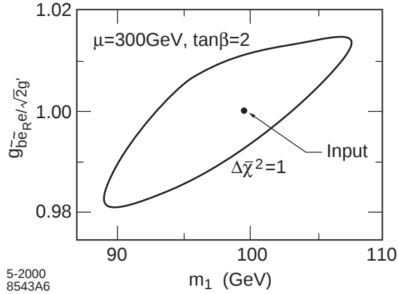
Figure 2.11: Determination of the g_{b\tilde{e}e} coupling from a 100 \text{ fb}^{-1} measurement of selectron pair production, from [80].
