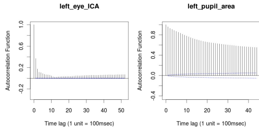
Figure 2: Auto-correlations for the ICA and pupil area.
