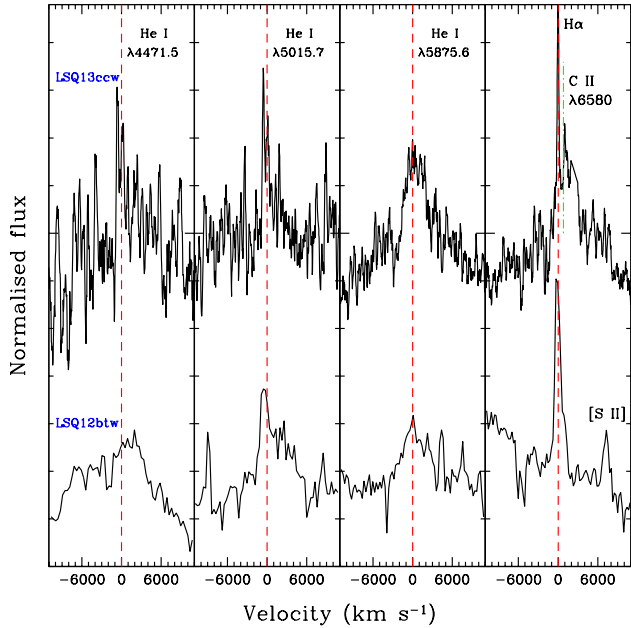
Figure 5. Profiles of three He I lines ( \lambda 4471 , \lambda 5016 , \lambda 5876 ) and the H\alpha region in the Keck-II spectrum of LSQ13ccw obtained on 2013 September 9, and in the NTT spectrum of LSQ12btw obtained on 2012 April 12. Dashed red vertical lines in the four panels mark the zero-velocity position of the He I and H\alpha lines; the dot-dashed green line in the right panel is centered at the average position of the C II \lambda\lambda 6578 , 6583 doublet.
