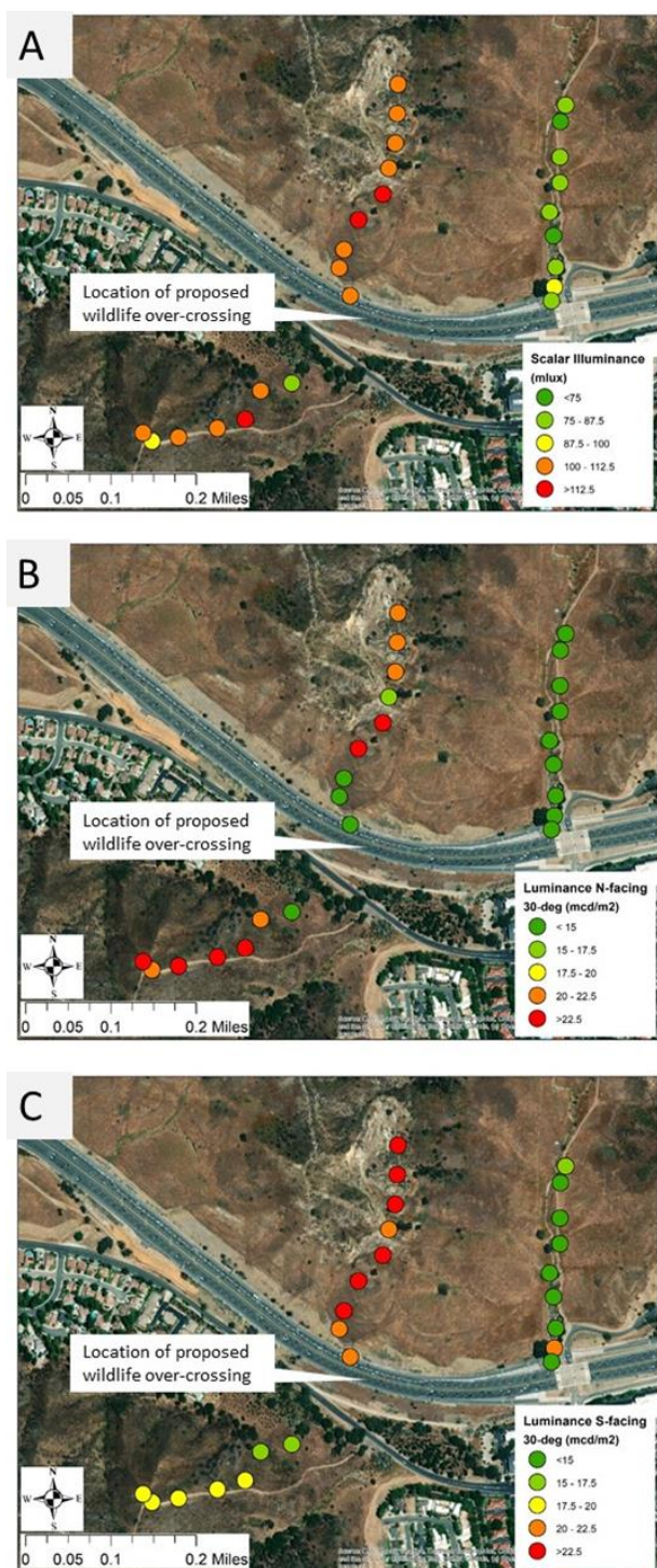
Figure 4. Light conditions along transects to the north and south of the proposed crossing site and along a creek bed east of the site, north of the highway. A) Scalar Illuminance (mlux); (B) Luminance (mcd/m 2 ) facing north from each point; and (C) Luminance (mcd/m 2 ) facing south from each point.
