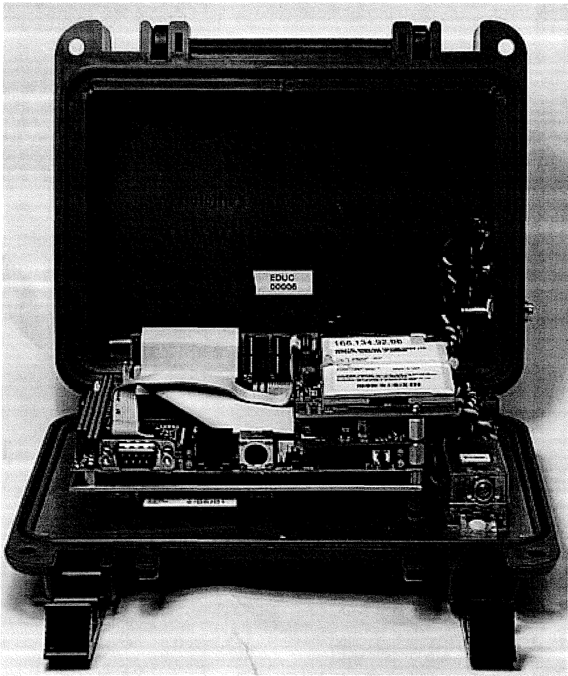
Figure 5. Final EDCU Design in R120 Case (interior view)
