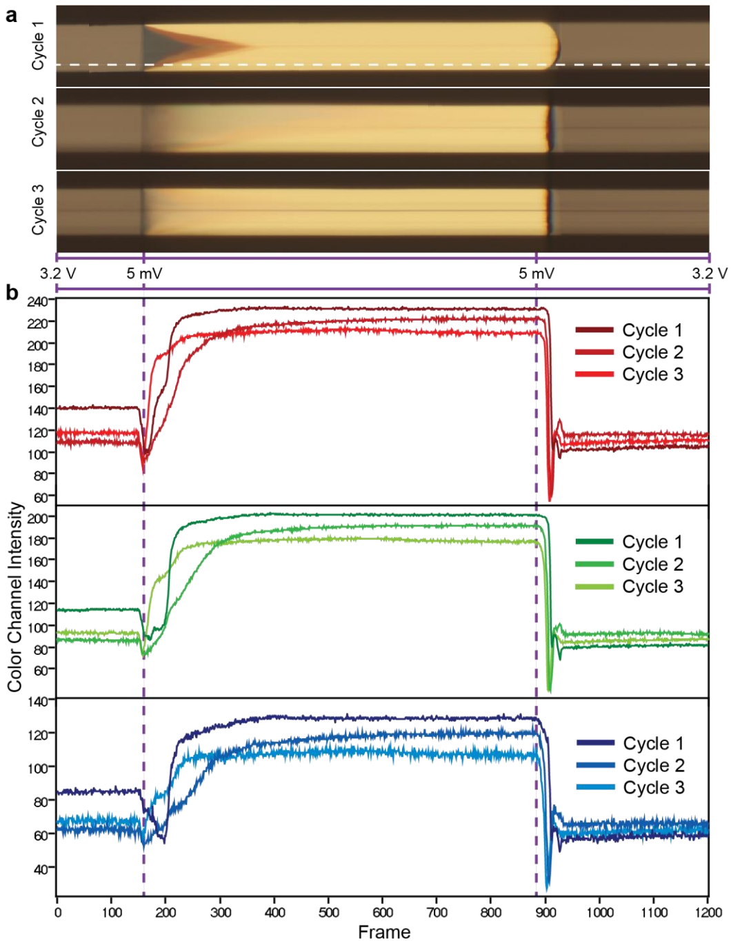
Figure S10. (a) Space-time slice of the first three lithiation/delithiation cycles. Movie S2 shows 2D (x,y) color maps as a function of time t . Here we display 2D (t, y) color maps. Each column here is a single-pixel column extracted from each frame in Movie S2 at the position indicated by the green arrow in Fig S9a. The three-phase coexistence and their constant velocity phase wavefronts are clearly seen in the first cycle, but absent in the following two cycles. The raw, unprocessed red, green, and blue (RGB) values for the dashed line profile in (a) is shown in (b) for all three cycles.
