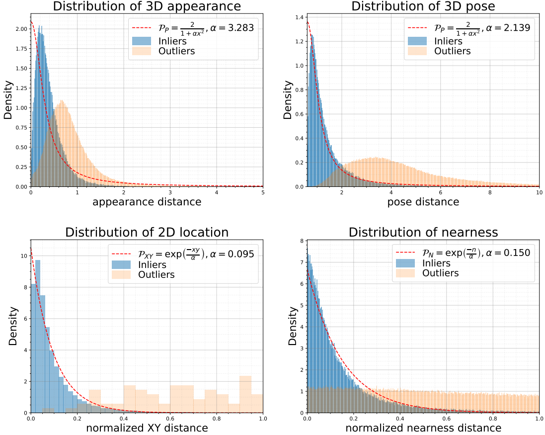
Figure 2.5: Conditional distributions of the attribute distances: We plot the data for the distances between the tracklet prediction and the single frame detection using annotated data from PoseTrack [3]. The curves show the distributions of correct matches (inliers) and incorrect matches (outliers). For 2D location and nearness the distances are normalized by the prediction interval.
