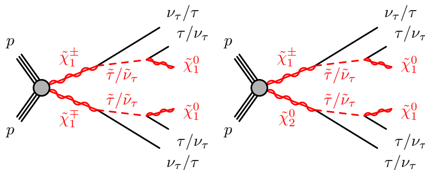
Figure 1: Representative diagrams for the electroweak production and decay processes of supersymmetric particles considered in this work: (left) \tilde{\chi}_1^+ \tilde{\chi}_1^- and (right) \tilde{\chi}_1^\pm \tilde{\chi}_2^0 production.
