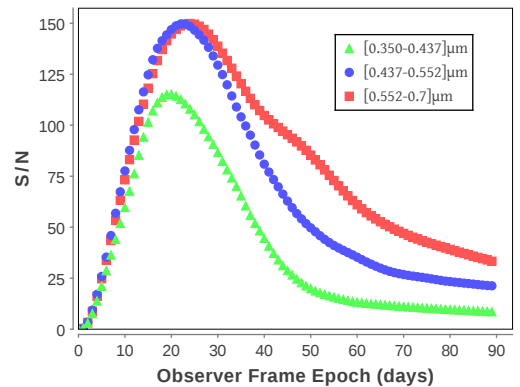
Figure 5: The signal-to-noise in three synthetic bands for a supernova at z = 0.08 : from [0.35\text{--}0.437] , [0.437\text{--}0.552] , and [0.552\text{--}0.7] \mu\text{m} based on the conditions given in Figure 4. The light curves are based on spectra taken every 24 hours with an exposure of 150 s.
