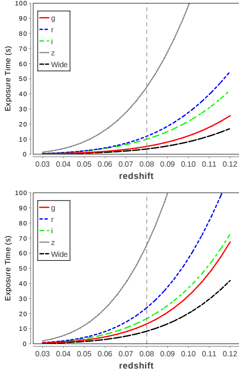
Figure 2: The exposure times required to obtain S/N = 5 ten days after explosion for a canonical supernova at AST3 using the Sloan g , r , i , z filters and a wide filter extending from 0.4\text{--}0.65\ \mu\text{m} . The figure on the left corresponds to a Galactic extinction of E(B - V) = 0.05 and the right to E(B - V) = 0.2 . Note that these plots have different ordinate ranges compared to those in Figure 1.
