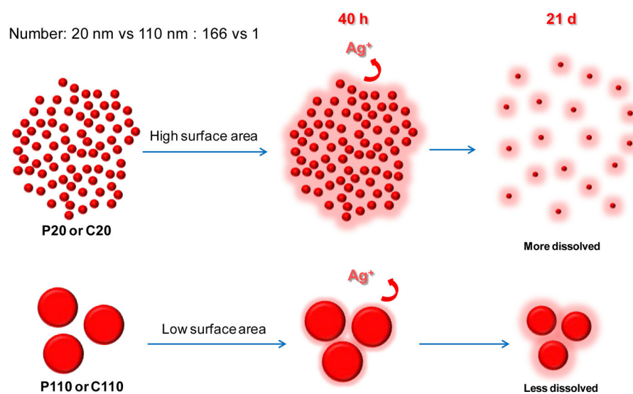
Figure 8. Schematic to explain the difference between the biological outcomes of exposure to 20 and 110 nm particles as a function of surface area and rates of dissolution.
