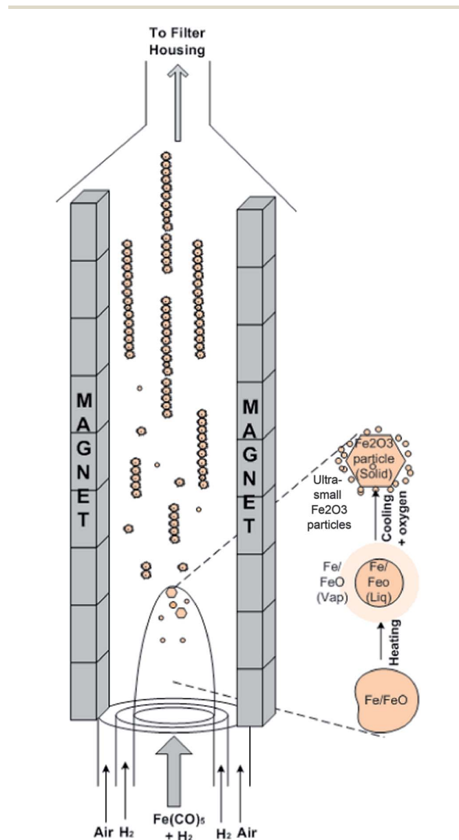
Fig. 1 Flame synthesis set-up. The magnified area shows different phases of iron oxide nanoparticles formation in different flame heights.
