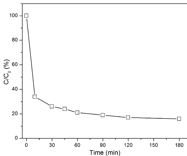
Fig. 6 Kinetics of adsorption of As(v) on the \gamma -Fe 2 O 3 nanochains at room temperature.
