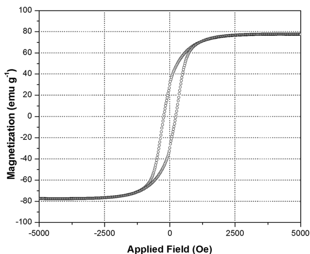
Fig. 5 Room temperature magnetic hysteresis loop of the γ-Fe 2 O 3 nanochains shows a saturation magnetism of 77 emu g -1 and coercivity of 290 Oe.
