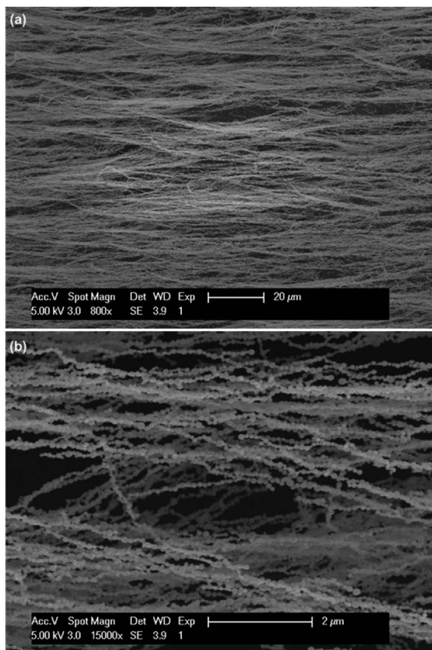
Fig. 2 (a) Large area SEM images of the ultra-long nanochains of iron oxides, (b) magnified view of the chains showing that each chain is made with thousands of nanoparticles forming a necklace-type structure.
