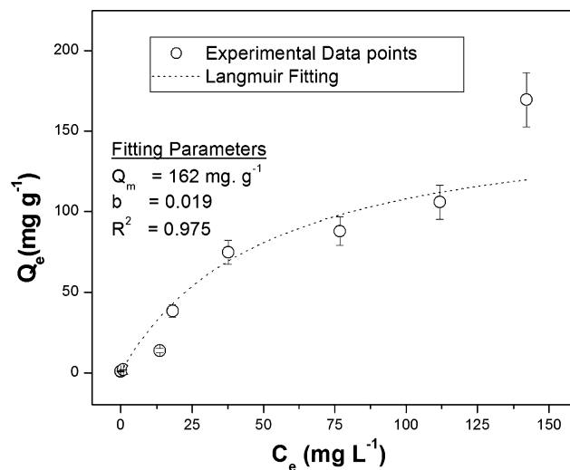
Fig. 7 Room temperature equilibrium isotherm data of As(v) adsorption on the \gamma -Fe 2 O 3 nanochains at pH = 7. Langmuir isotherm model was fit on to experimental data shown with the dotted line.
