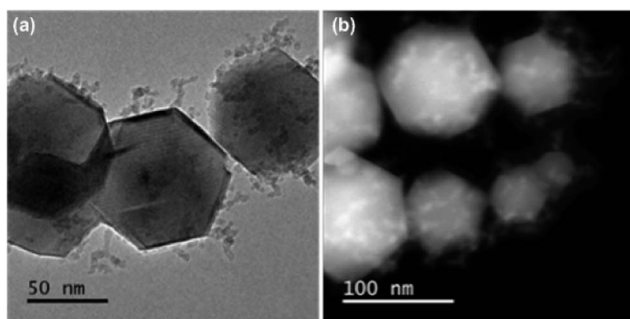
Fig. 3 (a) High resolution TEM image of individual nanoparticle of the chains show that they are covered with many ultra-small particles and dangling chains/clusters. (b) Annular dark field STEM image showing the morphology of the particles as well as the texture (heterogeneity) in the surface of the nanoparticles created by ultra-small particles.
