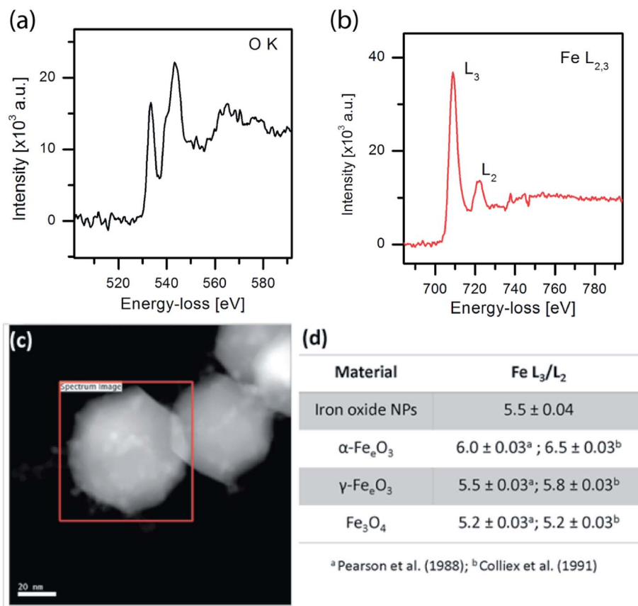
Fig. 4 EELS O K (a) and Fe L 2,3 (b) ionization edges acquired from the marked area of the HAADF STEM image in (c). The calculated Fe L 3 /L 2 EELS intensity ratio from (b) verified the γ-Fe 2 O 3 phase of the NPs when compared with reference values from the different oxidation states of iron oxide from the literature (d).
