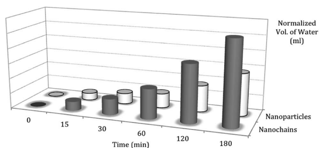
Fig. 8 The volume of water collected through the filters with nanochains, and nanoparticles as adsorbent materials at different time points. The bar graph shows a higher flow rate with nanochain-based filters than with an equivalent mass of nanoparticles.
