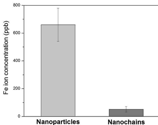
Fig. 9 The Fe ions detected by ICP-MS in water that was filtered through nanoparticles and nanochains at a fixed flow rate and a fixed total time.
