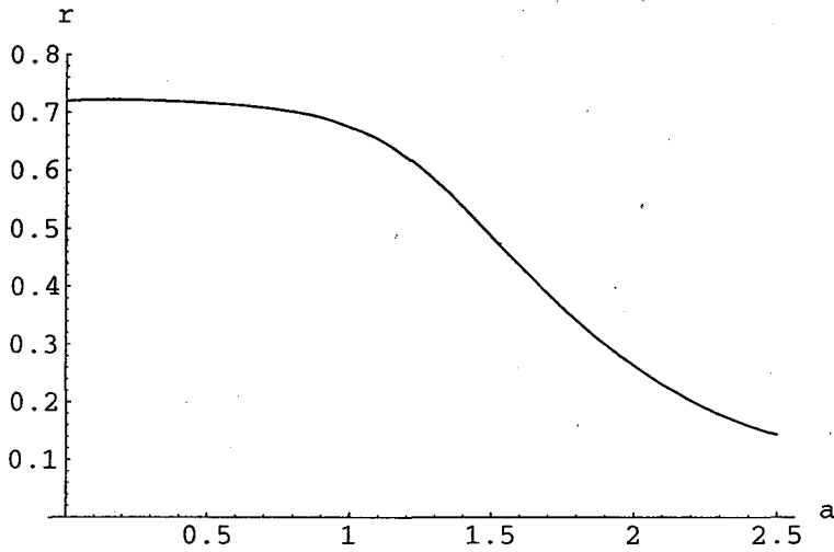
Figure 3.10: The mass ratio r of the lightest glueball to the KK mode on the compact D-brane coordinate \theta_2 along the generic direction a_1 = 2a_2 = a . Just as for the case with only one angular momentum, these states decouple very quickly from the spectrum.
