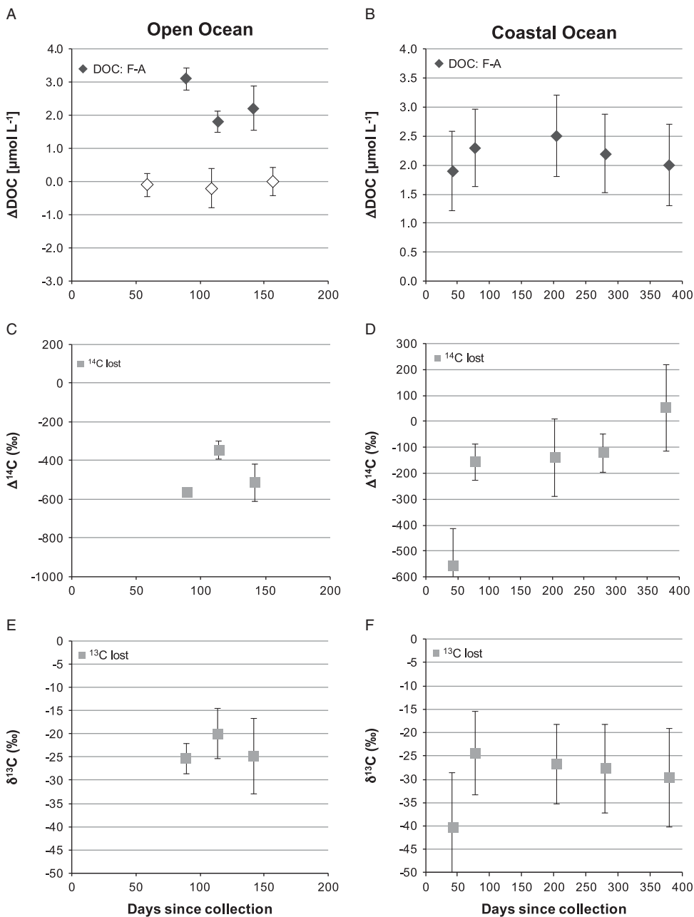
Figure 3 Comparison of Open vs. Coastal Ocean lost [DOC], \Delta^{14}\text{C} , and \delta^{13}\text{C} values. For all plots, error bars represent the propagated uncertainties of lost \Delta\text{DOC} , \Delta^{14}\text{C} , and \delta^{13}\text{C} values, determined via isotopic mass balance. Here, individual measurement uncertainties were used during error propagation (see Supplementary Material). In plots A–B, black diamonds represent \Delta\text{DOC} , offsets (frozen - acid) as in Figures 1–2. Open diamonds indicate acid/frozen duplicates with identical [DOC]. In plots C–F, squares represent determined \Delta^{14}\text{C} and \delta^{13}\text{C} values of DOC lost during acidified storage. In plots C and E, only half of the samples had \Delta\text{DOC} significantly different than zero; thus, we only report \Delta^{14}\text{C} and \delta^{13}\text{C} isotopic mass balance values for these n = 3 samples.
