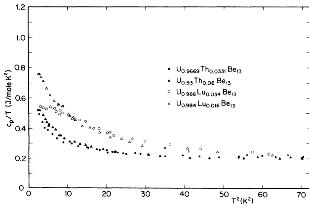
FIG. 1. c_p/T versus T^2 for various \text{U}_{1-x}\text{M}_x\text{Be}_{13} samples where M = \text{Th} and \text{Lu} , between 1.5 and 8.5 K.
