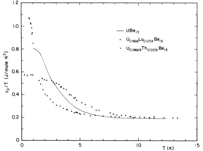
FIG. 2. Comparison of the influence of different impurities on the low-temperature normal-state specific heat of \text{UBe}_{13} .
