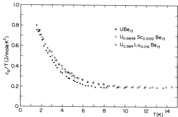
FIG. 3. Low-temperature normal-state specific heat of Lu- and Sc-doped \text{UBe}_{13} .
