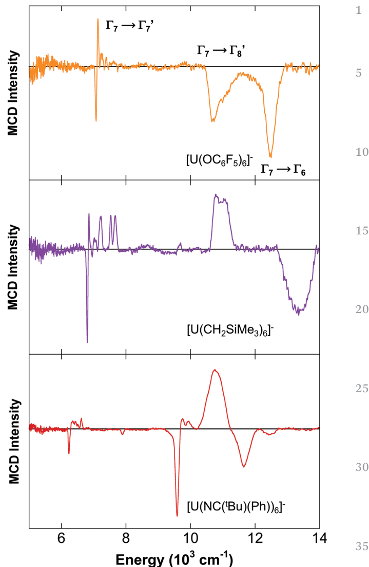
Fig. 3 The 5 K, 7 T NIR MCD spectra of top: [\text{U}(\text{OC}_6\text{F}_5)_6]^- , middle: [\text{U}(\text{CH}_2\text{SiMe}_3)_6]^- and bottom: [\text{U}(\text{NC}(\text{tBu})(\text{Ph}))_6]^- complexes.
