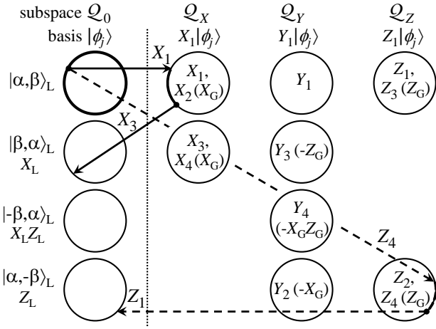
FIG. 4: State evolution and errors with continuous measurement. Thick-line circle illustrates diffusive evolution of the legitimate state [Eq. (39)] within 2-dimensional subspace of the gauge qubit due to measurement. The 12 single-qubit errors move the legitimate state to 8 other 2-dimensional subspaces in \mathcal{Q}_X , \mathcal{Q}_Y , and \mathcal{Q}_Z with the mapping described by Eq. (65) – see operators written inside the circles, the corresponding gauge qubit operations are in parentheses. If the second error occurs before the first error is detected (i.e., within the response time T_R ), it may move the state back to \mathcal{Q}_0 , so that both errors remain undetected (dotted line separates \mathcal{Q}_0 from error subspaces). Depending on a combination of the two errors, the logical qubit |\alpha, \beta\rangle_L may be affected by logical errors X_L , Y_L , or Z_L . The solid-line arrows illustrate a scenario of errors X_1 and X_3 , leading to logical error X_L ; the dashed-line arrows correspond to errors Z_4 and Z_1 , leading to Z_L .
