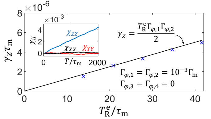
FIG. 6: (Color online) The rate \gamma_Z of the logical Z-error as a function of the response time T_R^e for the case when qubits 1 and 2 are subject to pure dephasing with \Gamma_{\varphi,1} = \Gamma_{\varphi,2} = 10^{-3}\Gamma_m . The crosses show numerical results, the solid line is the analytical result, Eq. (72). The inset shows the diagonal elements of the process matrix ( \chi_{XX} , \chi_{YY} , and \chi_{ZZ} ) as functions of time T for T_R^e = 20.8\tau_m . The rate \gamma_Z is calculated from the slope of \chi_{ZZ}(T) . We used \Theta = 1 , \eta = 1 , \tau_c = \tau_{c,opt} , and the exponential kernel for the correlators.
