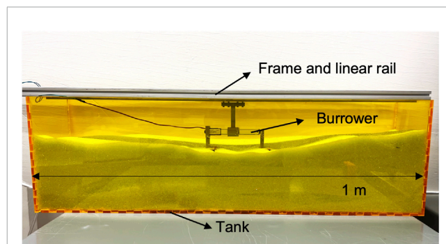
FIGURE 7 Granular bed for reciprocating burrower testing, with the burrower exposed for visualization.
