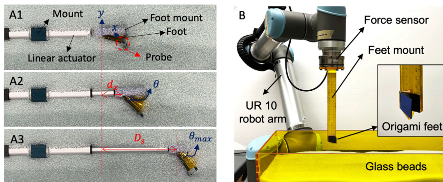
FIGURE 6 Experimental setup for single foot behavior (A) Tracking the deployment profile of a submerged foot (B) Experimental setup for measuring resistive force profile of the feet.
