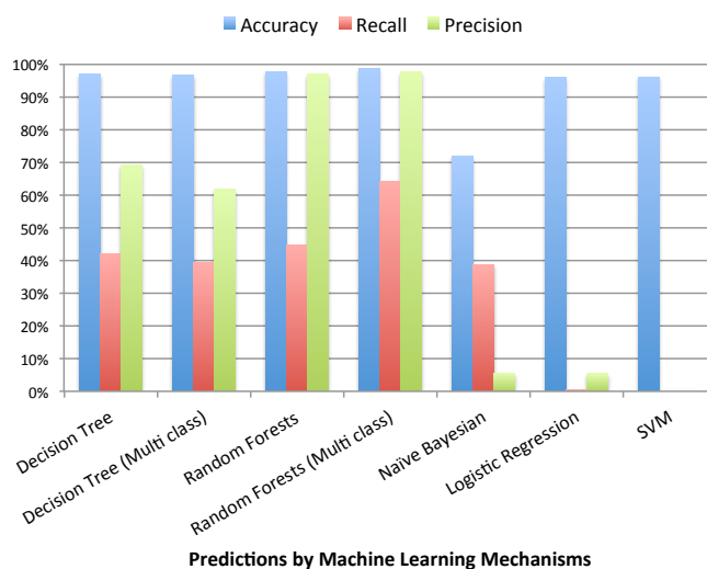
Fig. 3: Job status predictions by machine learning mechanisms
