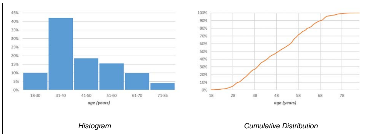
Figure 14. Distributions of respondents' age
