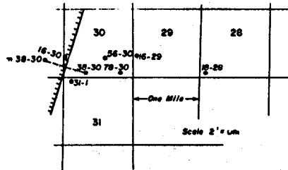
Fig. 9 - Inferred presence of a hydrologic barrier in the northern part of the East Mesa geothermal well field.
