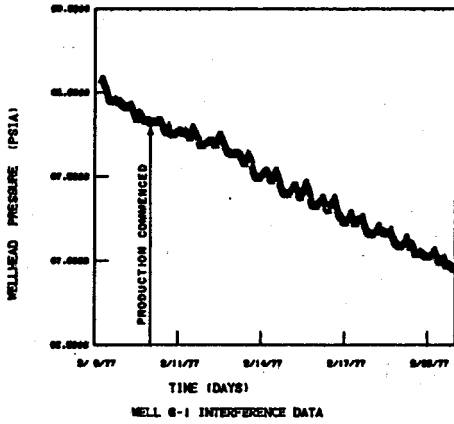
Fig. 6 - Wellhead pressures from well 6-1 with well 6-2 in production (~370m; 1,200 feet away).
