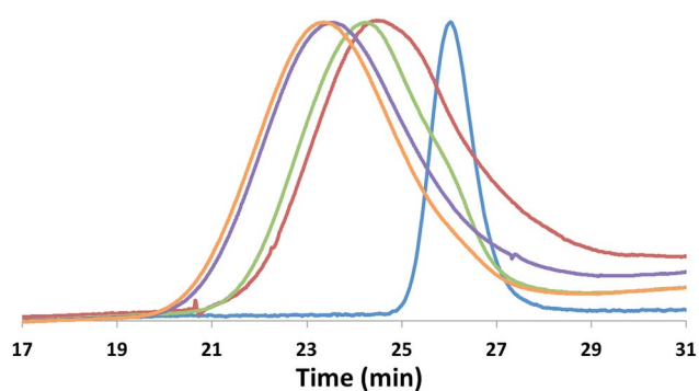
Fig. 8 SEC traces corresponding to the stepwise preparation of PLA- b -PTMC- b -PLA- b -PTMC- b -PLA ( M_n are reported in 10^3 \text{ g mol}^{-1} ; \mathcal{D} = M_w/M_n ): PLA (blue, M_n = 13.5 , \mathcal{D} = 1.09 ); PTMC- b -PLA (red, M_n = 20.0 , \mathcal{D} = 1.25 ); PLA- b -PTMC- b -PLA (green, M_n = 32.9 , \mathcal{D} = 1.29 ); PTMC- b -PLA- b -PTMC- b -PLA (purple, M_n = 40.0 , \mathcal{D} = 1.42 ); PLA- b -PTMC- b -PLA- b -PTMC- b -PLA (orange, M_n = 45.1 , \mathcal{D} = 1.43 ).
