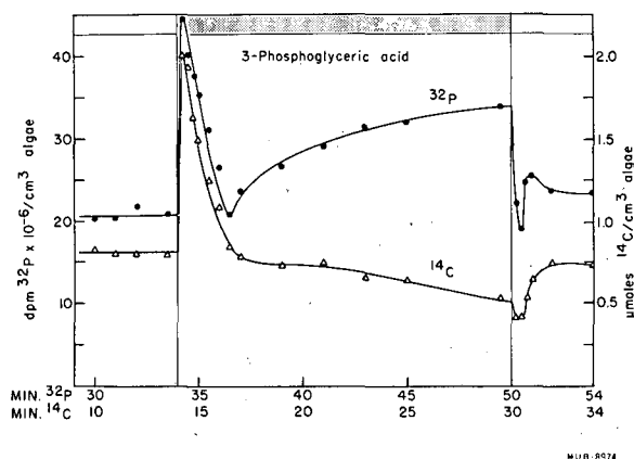
Fig. 1. Levels of ^{14}\text{C} - and ^{32}\text{P} -labeled PGA in Chlorella pyrenoidosa during photosynthesis and respiration.
