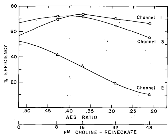
Fig. 4. Effect of choline reineckate on the efficiency of scintillation counting of ^{14}\text{C} in three channels. The scintillation mixture consisted of 16 ml of scintillation solution and 3 ml of acetonitrile containing 0, 8, 16, 32, and 48 \mu\text{M} of choline-reineckate. The channel settings were the same as indicated in Fig. 3.
