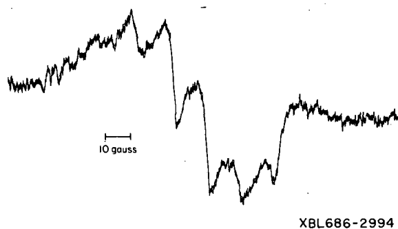
Fig. 3. ESR spectrum obtained on 1-hr H^\bullet irradiation of crystalline choline chloride.
