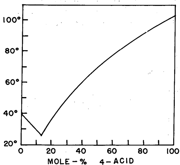
Fig. 4. (-)-1,2-Dithiane-3-carboxylic acid, and (-)-1,2-dithiane-4-carboxylic acid.
