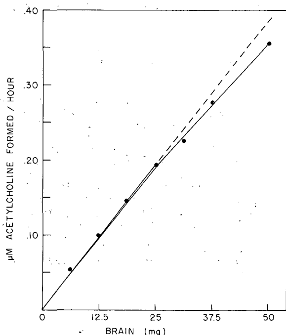
Fig. 2. Relation of ACh formation to amount of whole brain homogenate used. The standard incubation mixture ( 0.8 \text{ ml} ) was incubated with 0.8 \text{ ml} of rat brain homogenate. The rate of ACh formation was 8.1 \text{ } \mu\text{M/hr/g} . Data points are averages of duplicate analyses which agreed within 1\% .
