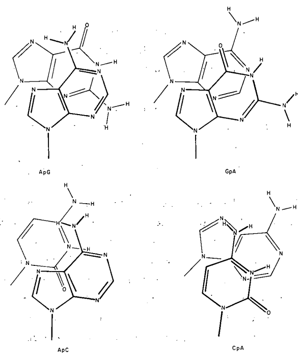
Fig. 13. Scale drawing of the bases in sequence isomers of dinucleoside phosphates assumed to have the geometry of a single strand of DNA. The pattern of groups available for hydrogen bonding are different.
