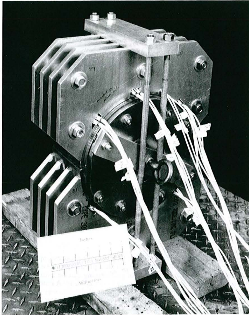
Fig. 1 The test setup. Aluminum plates clamp the shell pieces against the yoke for welding.
