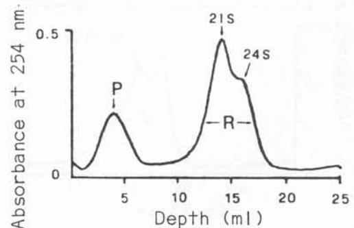
Fig. 3. Extinction profile in sucrose-density gradients of CVV-RNA released by the single-phase phenol system. Gradients were centrifuged 11 hours at 24,000 rpm in a Spinco SW 25.1 rotor. P = virus protein; R = RNA with 21 and 24 S components.
