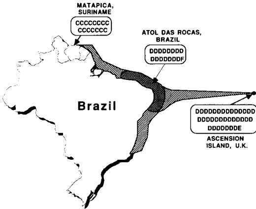
FIG. 4. MtDNA genotypes observed at the Ascension Island, Surinam, and Brazilian green turtle rookeries. Also shown (by cross-hatching) is the region of overlap on feeding grounds (as indicated by tag recoveries) for females that nest at the Ascension and Surinam rookeries (modified from Carr, 1975).
