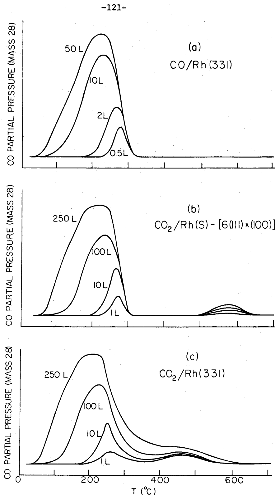
Figure III-32. TDS spectra from adsorption of (a) CO on Rh(331), (b) CO 2 on Rh(S)-[6(111) × (100)] and (c) CO 2 on Rh(331). The only species detected desorbing in all three cases was CO.
