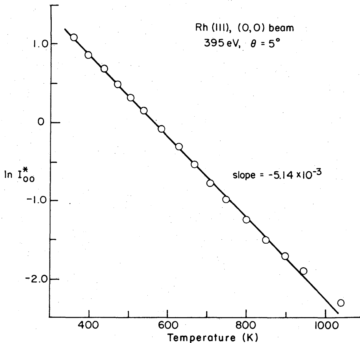
Figure III-5. A plot of \ln I_{00}^* vs temperature for the specular \ell = 7 Bragg peak from the Rh(111) surface.
