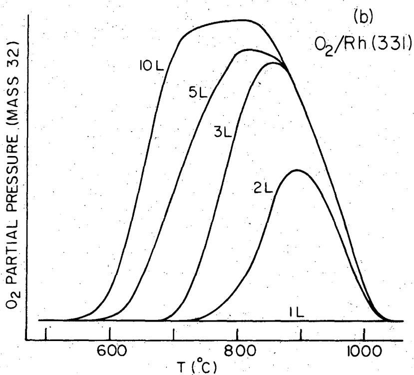
Figure III-29. TDS spectra from oxygen adsorption on (a) Rh(S)-[6(111)\times(100)] and (b) Rh(331) .
