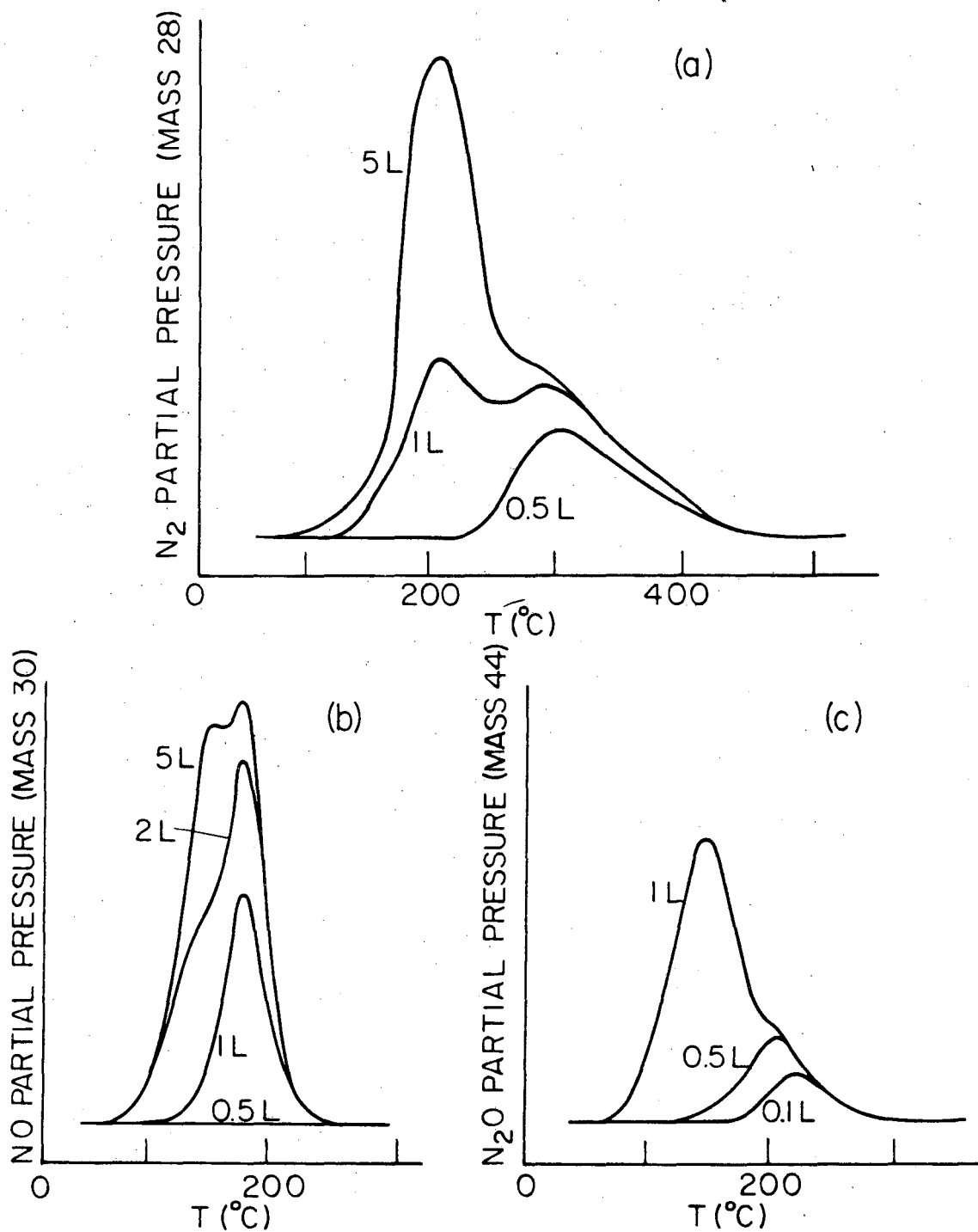
Figure III-34. TDS spectra obtained from NO adsorption on Rh(S)-[6(111)×(100)]. (a) N 2 desorption, (b) NO desorption and (c) N 2 O desorption.
