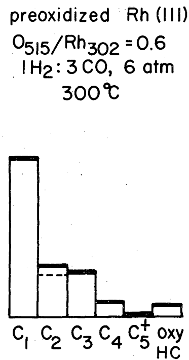
Figure III-51. Product distribution, in weight percent, after 2 hours of CO hydrocarbon over pretreated Rh(III) crystals. The areas above and below the dotted line in the C 2 fraction represent the amount of ethane and ethylene, respectively. Oxy HC is the sum of the CH 3 OH, CH 3 CH 2 OH and CH 3 CHO fractions.
