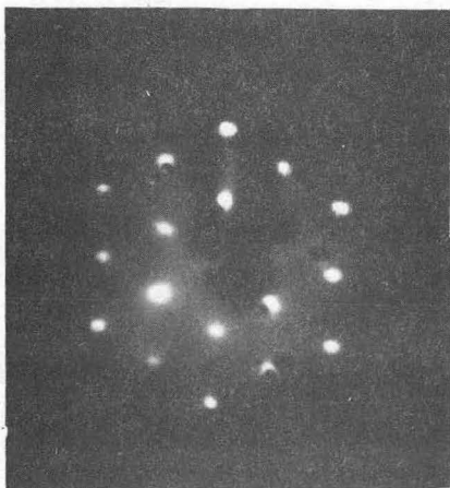
Figure III-18. LEED patterns formed by NO adsorption on the Rh(111) surface.
