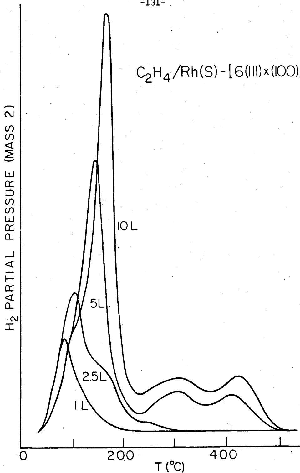
Figure III-35. (a) Hydrogen desorption from C 2 H 4 adsorption on Rh(S)-[6(111)x(100)].
