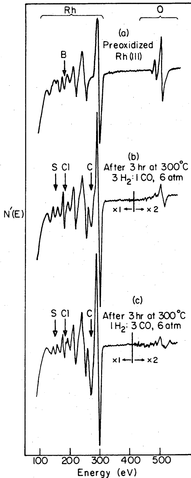
Figure III-48. AES spectra from a preoxidized Rh(III) crystal. (a) before a reaction O_{515}/Rh_{302} = 0.6 , (b) after a 3 hour reaction of a 3H_2:1CO gas mixture at 300° and 6 atm, and (c) after 3 hour reaction of a 1H_2:3CO gas mixture at 300°C and 6 atm.
