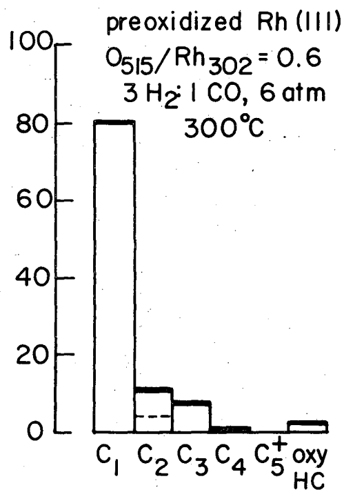
Figure III-51. Product distribution, in weight percent, after 2 hours of CO hydrocarbon over pretreated Rh(III) crystals. The areas above and below the dotted line in the C 2 fraction represent the amount of ethane and ethylene, respectively. Oxy HC is the sum of the CH 3 OH, CH 3 CH 2 OH and CH 3 CHO fractions.
