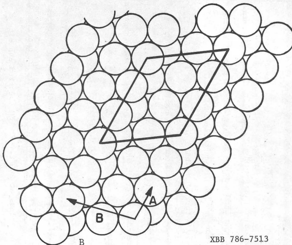
Figure III-33. (a) LEED pattern of \text{Rh}(331)-\begin{pmatrix} -1 & 1 \\ 3 & 0 \end{pmatrix} structure at 44 eV. (b) Real space unit cell of \begin{pmatrix} -1 & 1 \\ 3 & 0 \end{pmatrix} structure. A and B are \text{Rh}(331) unit cell vectors.
