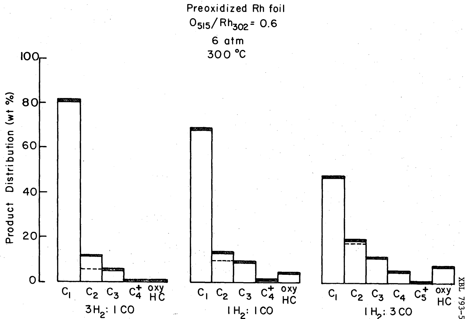
Figure III-57. Product distribution, in weight percent, after 2 hours of CO hydrogenation over preoxidized Rh foil. The areas above and below the dotted line in the C 2 fraction represent the amount of ethane and ethylene, respectively. Oxy HC is the sum of the CH 3 OH, CH 3 CH 2 OH and CH 3 CHO fractions.
