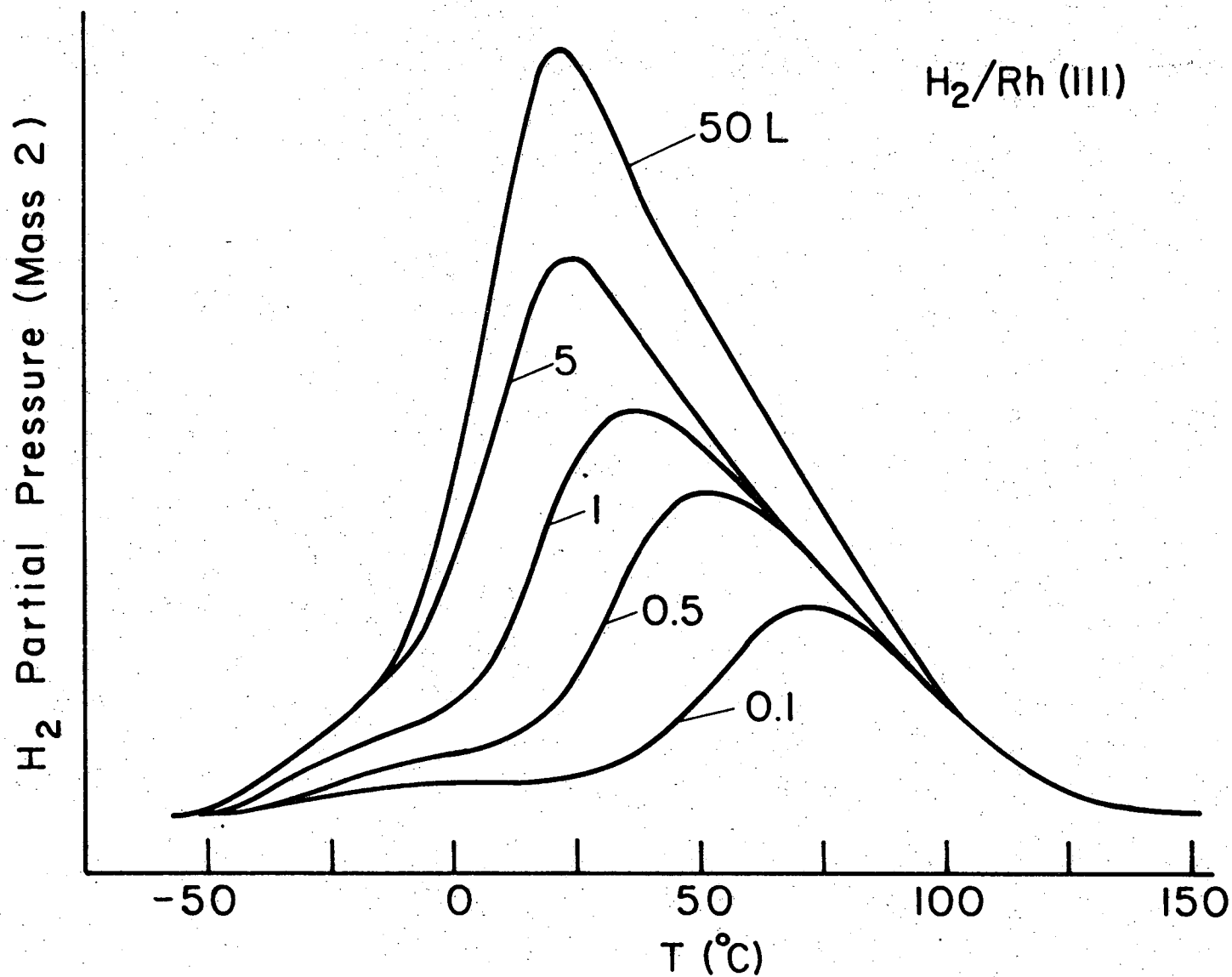
Figure III-8. Thermal desorption spectra obtained from adsorbing 0.1 to 50 L of hydrogen on Rh(III).
