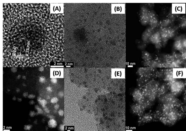
Fig. 2 TEM images of 1C and 2B . (A) Lattice-resolved image of one of the particles of 1C ; (B) distribution of \text{Ta}_x\text{N}_y NPs on silica in 1C ; (C) dark field STEM image showing the dispersion of the NPs in 1C ; (D) high-magnification dark field STEM image of 2B showing the NPs; (E) NPs in 2B ; and (F) low magnification dark-field STEM image of 2B .
