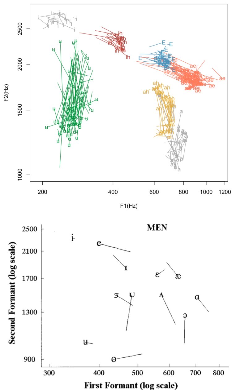
Figure 3.6: Top: Vowel trajectories for a speaker of California English. Each line segment represents one vowel produced by this speaker. Formants at vowel onset are at the unlabeled end of the line segment, and formants at vowel offset are at the labeled end of the line segment. Bottom: Trajectories of midwestern American English vowels, as reported by Hillenbrand and Nearey (1999).
