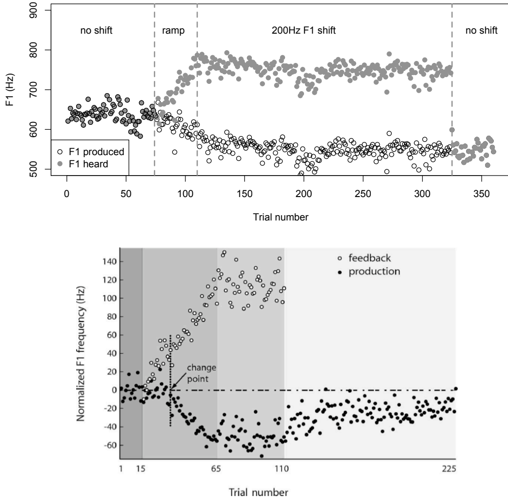
Figure 3.5: Top: Change in F1 feedback and F1 production in / \epsilon / over the course of the experiment for a representative subject. Gray filled circles mark the F1 values that the subject heard at each trial. Open circles mark the F1 that the subject produced at each trial. Thus, each gray circle/open circle pair represents one trial. Bottom: Change in F1 feedback and F1 production in / \epsilon / over the course of the experiment, averaged across subjects from Purcell & Munhall, 2006. Open circles indicate the F1 values that the subject heard at each trial, and black filled circles mark the F1 that the subject produced at each trial.
