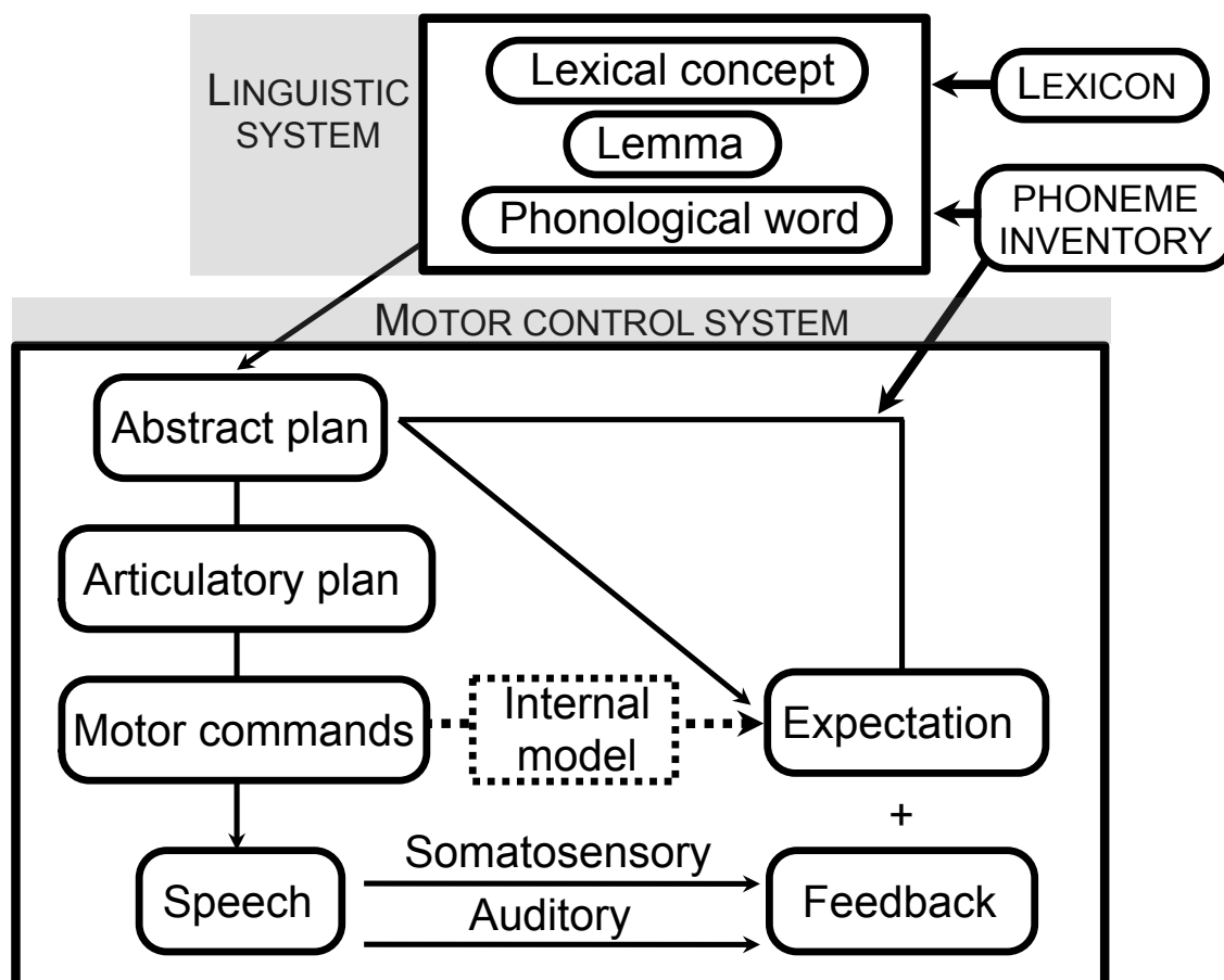
Figure 7.1: Unified model of speech production.
