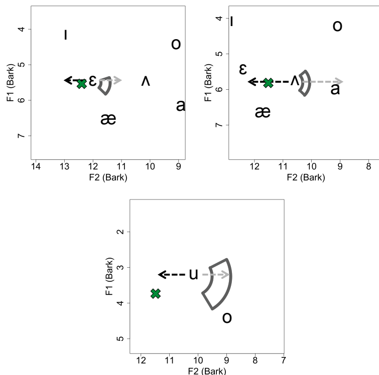
Figure 5.8: Green “x” shows the mean formants heard during the maximum F2 feedback shift in /ε/ (top left); /Λ/ (top right); /u/ (bottom). Formants were normalized with the magnitude-angle method described above. Wedges display the 25th and 75th percentiles of compensation magnitudes and angles during these trials.
