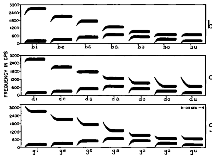
Figure 2.1: Vowel formant transitions in American English. From Delattre, Liberman, & Cooper, 1955.
