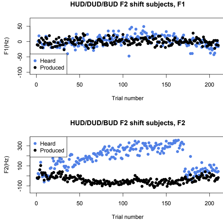
Figure 5.5: Response to / \Lambda / F2 feedback shift. The x-axis marks the trial number. Blue dots mark the normalized formant that the talkers heard, on average, at each trial. Black dots show the formants they produced at each trial, on average. The top graph shows F1 over the course of the experiment, and the bottom graph shows how subjects compensate for a shift in / \Lambda / F2. See text for normalization procedure.
