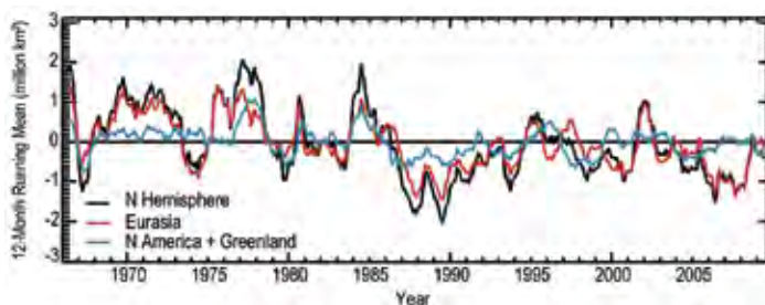
FIG. 2.21. Twelve-month running anomalies of monthly snow cover extent over Northern Hemisphere land (including Greenland) as a whole and Eurasia and North America separately between Nov 1966 and Dec 2010. Anomalies are calculated from NOAA snow maps. Mean hemispheric snow extent is 25.0 million km 2 for the full period of record. Monthly means for the period of record are used for nine missing months between 1968 and 1971 in order to create a continuous series of running means. Missing months fall between June and October; no winter months are missing.
