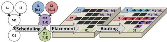
Fig. 6. Illustration of a typical compiler targeting a DMFB: the protocol to execute is represented as a DAG. The compiler must schedule, place, and route all operations in order to produce an executable sequence of electrode activations to automatically run the protocol.
