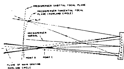
Fig.4. Bartoe segmented predisperser (1974).
