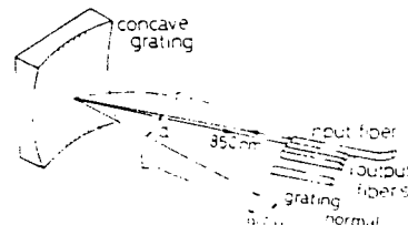
Fig. 10. Optical de-multiplexer using a VLS grating. From Kita & Harada (1983).
