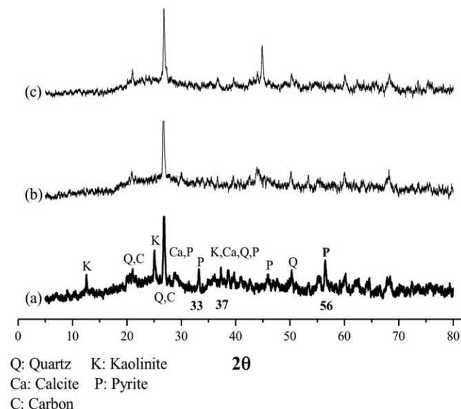
Fig. 6. XRD patterns of (a) unprocessed lignite, (b) pyrolysis char, and (c) hydropyrolysis char of Tuncbilek lignite.
