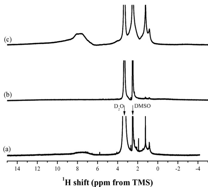
Fig. 7. Liquid ^1\text{H} NMR spectra of the components extracted in DMSO of (a) unprocessed Tuncbilek lignite, (b) its pyrolysis char, and (c) its hydropyrolysis tar.
