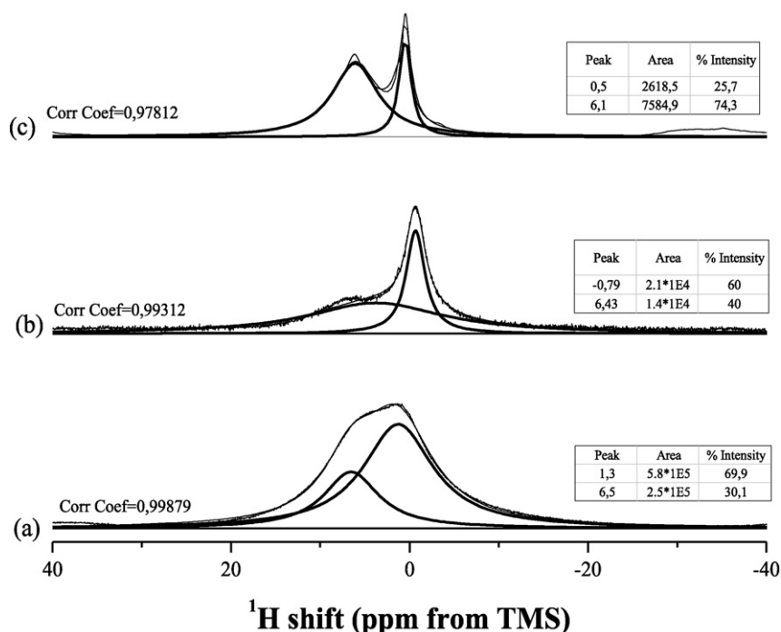
Fig. 4. 1 H NMR spectra of (a) unprocessed Tuncbilek lignite, (b) its pyrolysis char, and (c) its hydropyrolysis tar.
