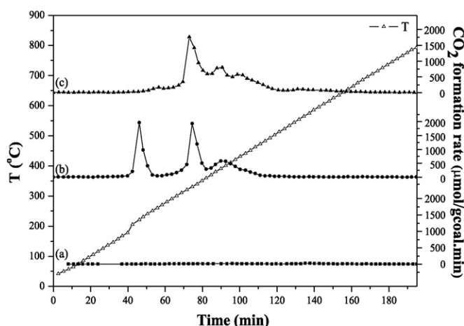
Fig. 3. Comparison of CO 2 formation rate during pyrolysis (a), oxidation of parent coal (b), and oxidation of pyrolysis char (c).
