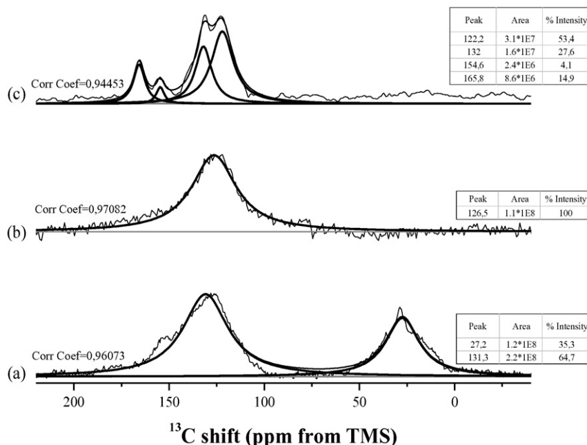
Fig. 5. ^{13}\text{C} (CP) MAS NMR spectra of (a) unprocessed Tuncbilek lignite, (b) its pyrolysis char, and (c) its hydropyrolysis tar.
