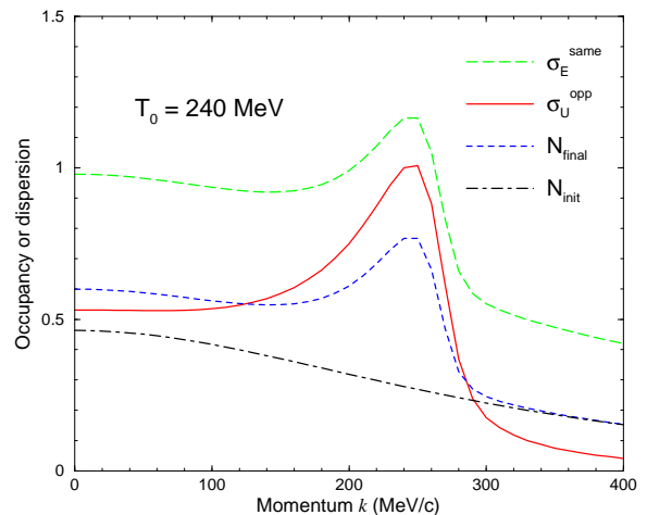
FIG. 1. The amplification and correlation obtained for an idealized spatially constant mass function \mu(t) emulating an expanding scenario that starts from an environment in which the order parameter is \sigma_0 \approx 26 MeV (corresponding to T_0 \approx 240 MeV). Further explanation is given in the text.
