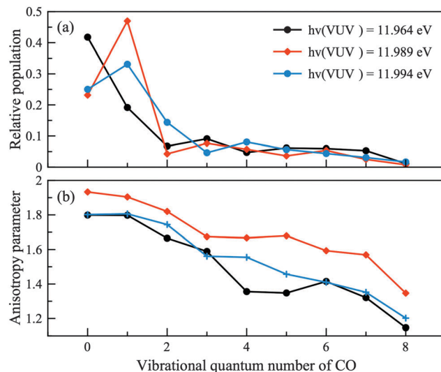
Fig. 5 (a) Comparison of the relative vibrational state populations of CO(X^1\Sigma^+; v = 0-8) at CO_2 photodissociation energies of 96495.7\text{ cm}^{-1} (11.964 eV) in black, 96697.5\text{ cm}^{-1} (11.989 eV) in red, and 96738.8\text{ cm}^{-1} (11.994 eV) in blue. (b) Comparison of the \beta parameters for individual CO(X^1\Sigma^+; v = 0-8) vibrational states transformed from the O(^1S) VMI-PI images at CO_2 photodissociation energies of 96495.7\text{ cm}^{-1} (11.964 eV) in black, 96697.5\text{ cm}^{-1} (11.989 eV) in red, and 96738.8\text{ cm}^{-1} (11.994 eV) in blue.
