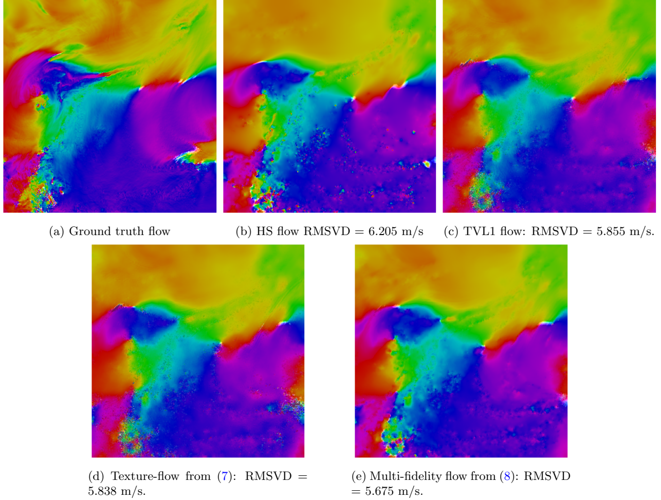
Figure 5: Colored flow visualization of extratropical cyclone (ETC) data.
