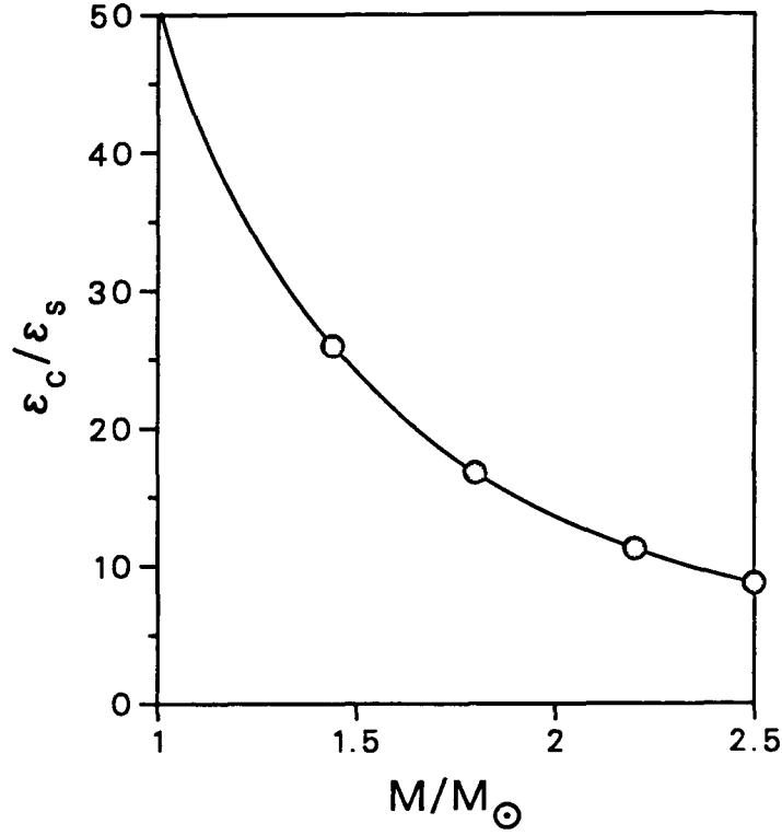
Figure 3: Central energy density in units of normal nuclear saturation density for the non-rotating neutron stars whose rotating counterparts have the shortest possible Kepler period, namely those corresponding to Fig. 1.
