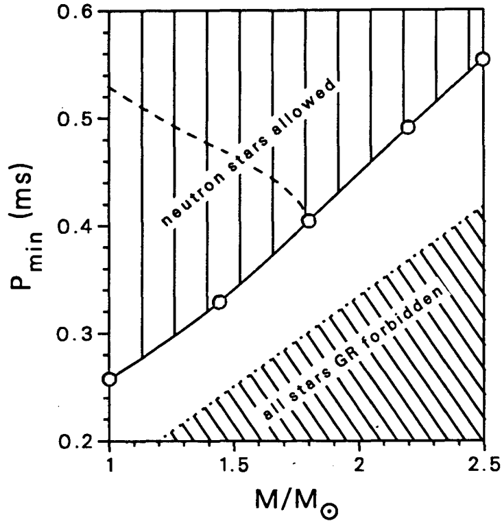
Figure 1: Minimum rotational period of neutron stars - solid curve. Calculated points are shown by dots. Periods of a sequence of stars whose maximum mass is 1.8M_{\odot} - dashed line. Region forbidden by structure of general relativity (modulo the approximate formula eq. (5)) - diagonal shaded region.
