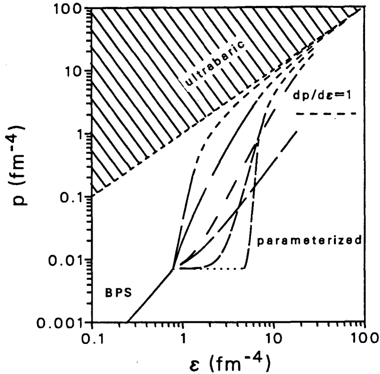
Figure 2: Bottom two equations of state produce minimum rotational period for a 1.442M_{\odot} neutron star, one with condensate ( p = \text{const.} region) and the other without. Others illustrate the flexibility of the simplest parameterization, eqs. (2-4). The three segments of each are (a) BPS, (b) parameterized region, (c) causal limit, dp/d\epsilon = 1 . Ultrabaryonic region has p > \epsilon . Its boundary is p = \epsilon . This region is inaccessible from below when dp/d\epsilon \leq 1 .
