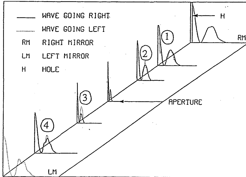
Figure 4: Calculated intra-cavity mode profile for the left and right propagating wavefronts. The number next to some of the profiles denotes the corresponding experimental profile at that location shown in Fig. 3.
