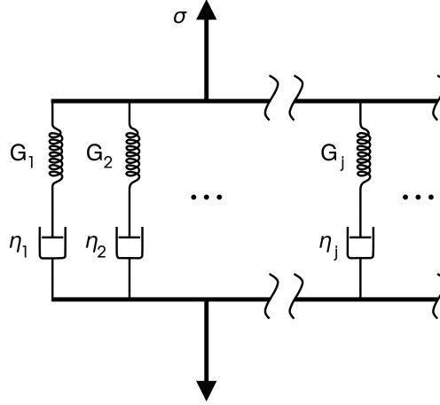
Figure 7.1: Spring-Dashpot analog for the linear viscoelastic multi-stage generalized Maxwell fluids
