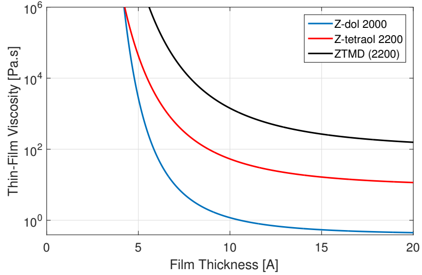
Figure 6.1: viscosity \eta(h) as a function of lubricant thickness h at room temperature T = 25^\circ\text{C} for Z-dol 2000 [15], Z-tetraol 2200, and ZTMD [41].
