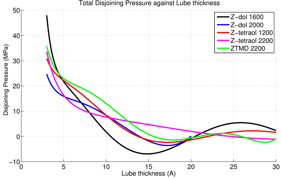
Figure 4.2: Total (sum of dispersive and polar components) disjoining pressure as a function of lubricant thickness for Z-dol 1600, Z-dol 2000, Z-tetraol 1200, Z-tetraol 2200, and ZTMD. It is noticeable that ZTMD and Z-tetraol 1200 have a close disjoining pressure and critical lubricant thickness (where d\Pi/dh = 0 ). This graphs are obtained according to Eq. 4.7 differentiating the surface energy function with respect to the lubricant thickness.
