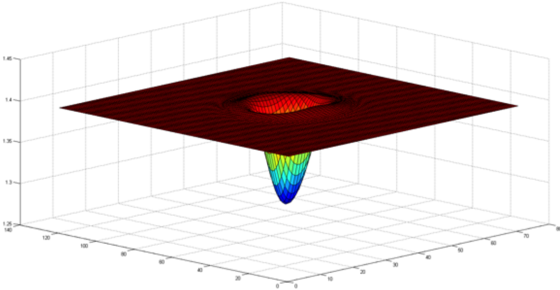
Figure 5.1: An example of the lubricant depletion including trough and side ridges for a typical laser shine condition of 2ns illumination with 20nm laser spot and 350^\circ C peak temperature of the spot.
