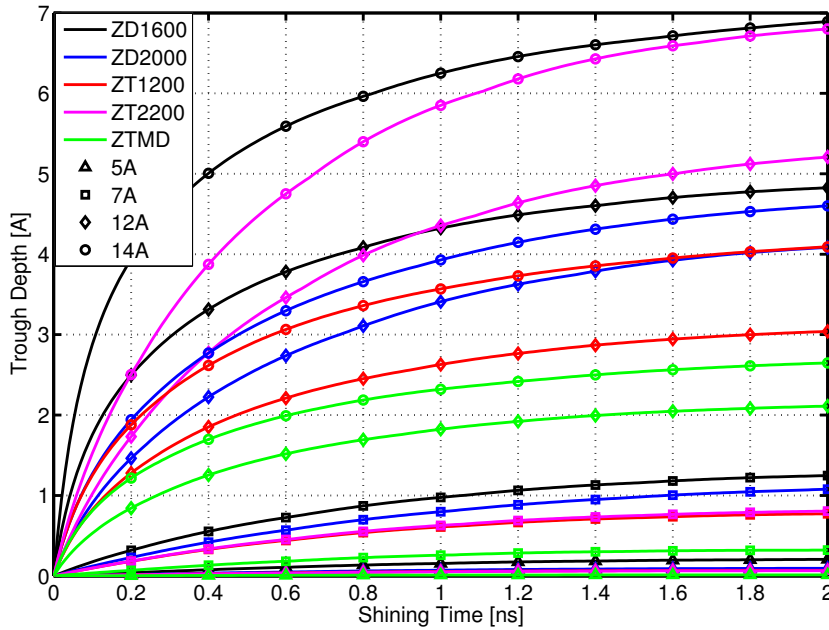
Figure 5.7: Trough depth versus time for different lubricants (different colors) and different initial lubricant thicknesses (different markers).
