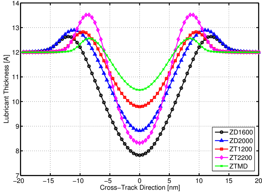
Figure 5.4: Final lubricant thickness profile for different lubricants at 12\text{\AA} initial lubricant thickness ( h_0 = 12\text{\AA} ) after 2ns of laser shine. Z-tetraol 2200 exhibits a huge deformation due to its weak film stiffness (low disjoining pressure derivative)
