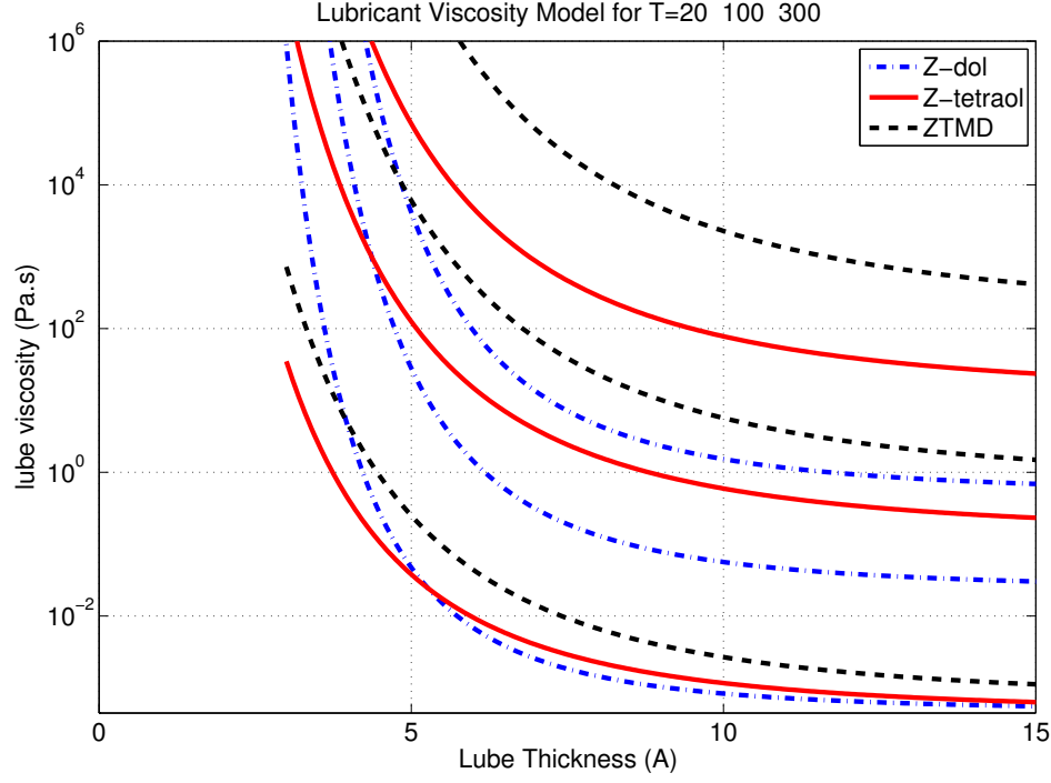
Figure 4.4: Thin-film effective viscosity as a function of lubricant thickness for different temperatures for different lubricants. For each lubricant, 3 graphs are plotted corresponding to viscosity as a function of temperatures: T = \{20, 100, 300^\circ\text{C}\} . Higher curves correspond to lower temperatures (closer to room temperature)
