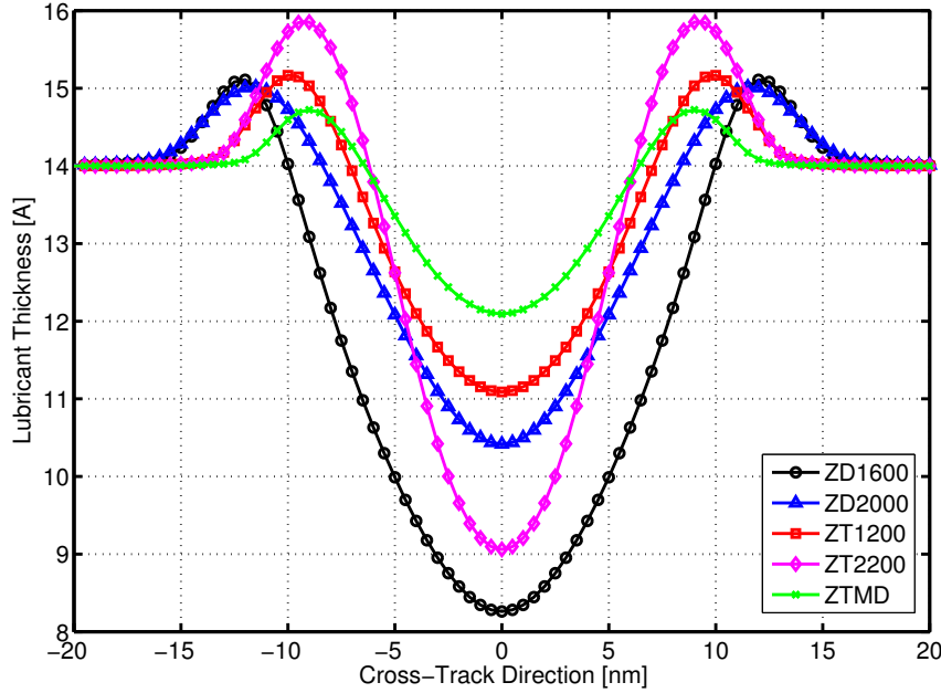
Figure 5.5: Final lubricant thickness profile for different lubricants at 14Å initial lubricant thickness ( h_0 = 14\text{\AA} ) after 2ns of laser shine.
