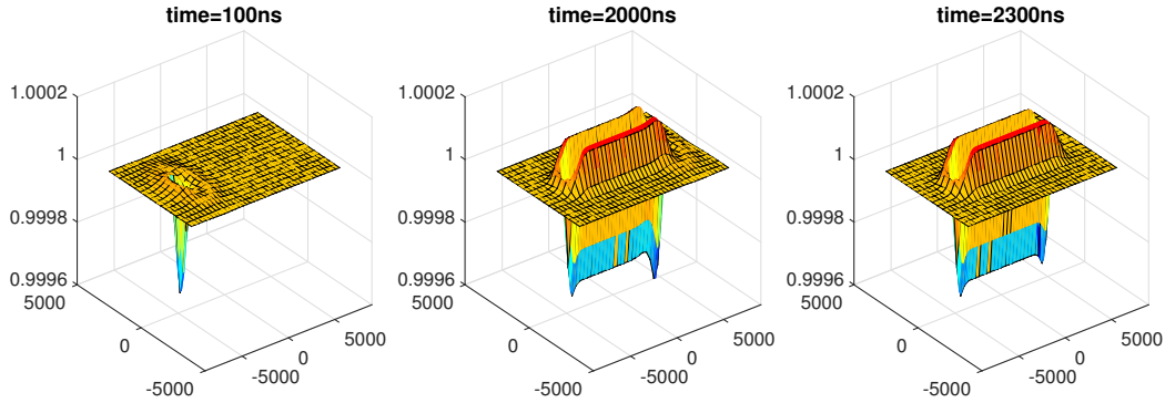
Figure 10.6: Viscoelastic FEA results for lubricant deformation and a laser spot size of L = 2\mu m a) right after the laser exposure, b) after a 2\mu s period, c) right after the laser exposure ends
