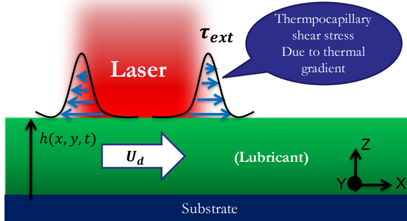
Figure 2.2: A schematic illustration of the lubricant under HAMR conditions.
