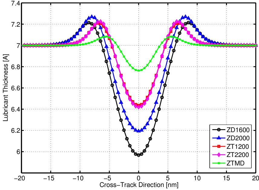
Figure 5.3: Final lubricant thickness profile for different lubricants at 7Å initial lubricant thickness( h_0 = 7\text{\AA} ) after 2ns of laser shine. The profiles of Z-tetraol 1200 and 2200 nearly coincide.
