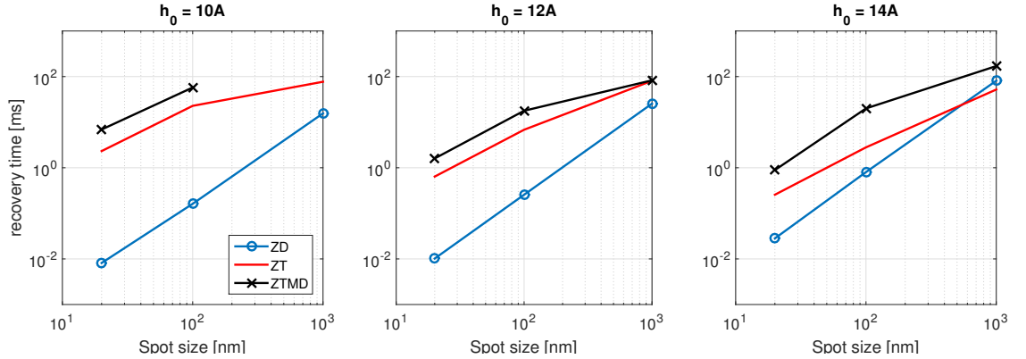
Figure 6.5: The recovery time as a function of the laser spot size for different lubricants different initial film thicknesses of h_0 = 1.0, 1.2, 1.4nm
