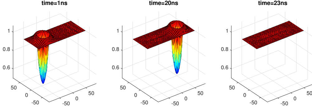
Figure 10.4: Viscoelastic FEA results for lubricant deformation and a laser spot size of L = 20nm a) right after the laser exposure, b) after a 20ns period, c) right after the laser exposure ends
