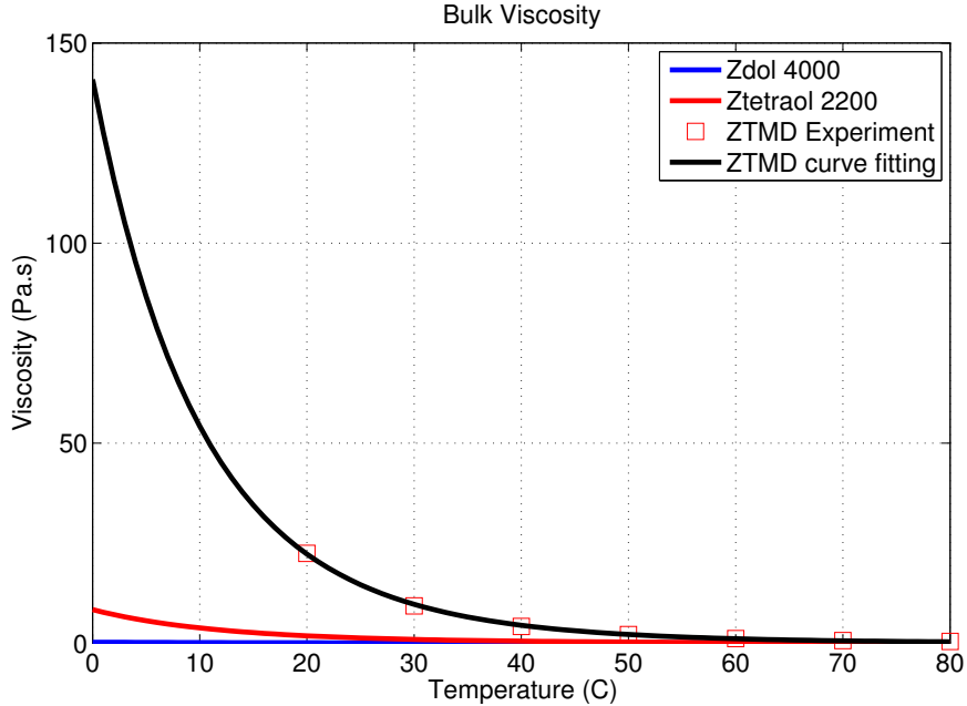
Figure 4.3: Bulk viscosity as a function of temperature for 3 different type of lubricants including Z-dol, Z-tetraol and ZTMD. It is clear that ZTMD has a greater viscosity compared to Z-tetraol and Z-tetraol compared to Z-dol.
