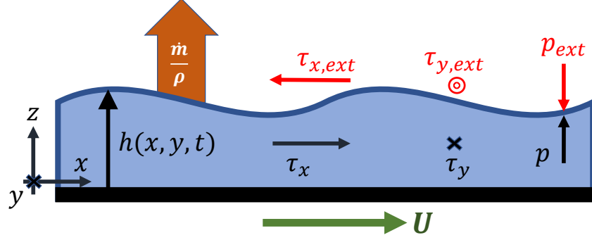
Figure 3.1: HAMR lubricant write process schematic: Lubricant flow is driven by the resulting external thermo-capillary shear stresses (\tau_{x,ext}, \tau_{y,ext}) and the pressure gradient (\nabla p)_{ext} . Some lubricant is also removed from the film via mass evaporation \dot{m} . The thin lubricant film of unknown thickness h(x, y, t) is subjected to a scanning laser spot of speed U , which is represented by a prescribed Gaussian temperature distribution T(x, y, t) , as shown in Fig. 2.2.
