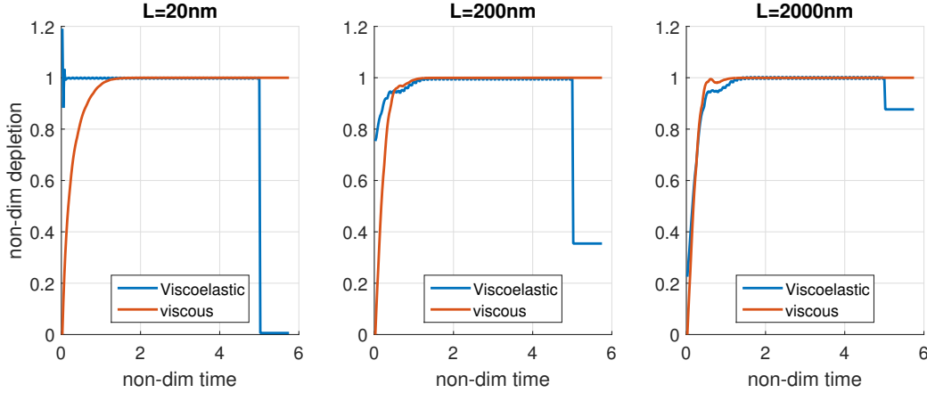
Figure 10.7: Time history of the depletion for 3 laser spot sizes of L = 20nm, 200nm, 2\mu m . In each plot the results of the viscoelastic FEA are compared to the case of the viscous lubricant where the viscoelastic effects are suppressed. The time is normalized by the timescale and depletion by maximum depletion of each case.
