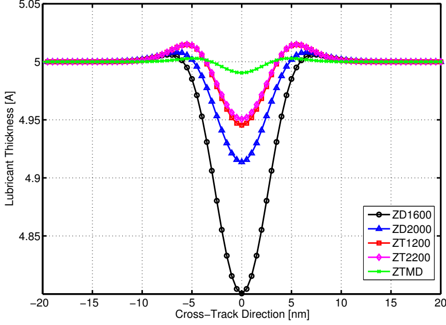
Figure 5.2: Final lubricant thickness profile for different lubricants at 5Å initial lubricant thickness( h_0 = 5\text{\AA} ) after 2ns of laser shine.
