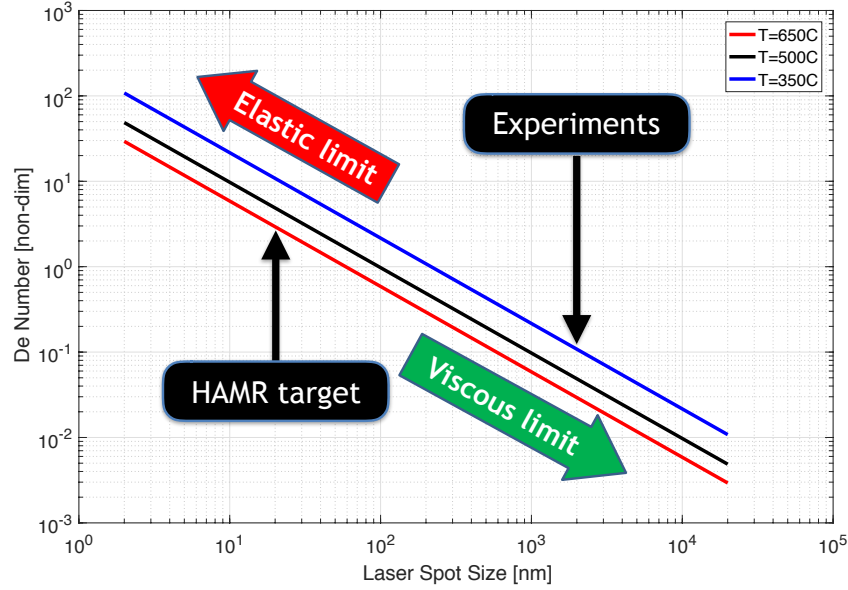
Figure 8.3: Deborah number as a function of laser spot size L , for different HAMR peak temperatures of T = 350, 500, 650^\circ\text{C} , for Z-tetraol 2000 and disk speed of U = 5\text{m/s}
