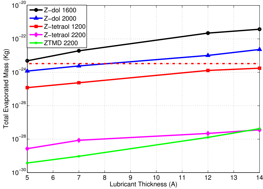
Figure 5.6: Evaporation as a function of lubricant thickness for different lubricants. As the lubricant thickness increases, the amount of evaporation also increases since the lube bonding ratio decreases. ZTMD and Z-tetraol 2200 exhibit much less evaporation due to their smaller bulk evaporation pressure. The red dashed line represents the mass of a typical molecule with M_w = 2000Da
