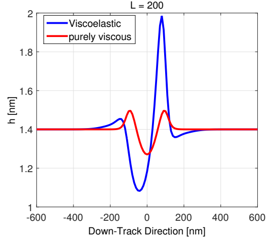
(b) Laser spot size L = 200nm
