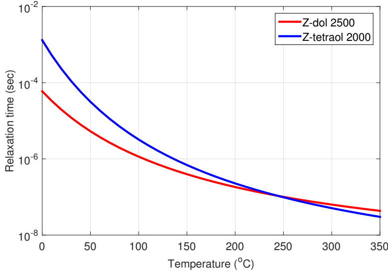
Figure 7.2: Maxwell relaxation time as a function of temperature for Z-dol 2500 and Z-tetraol 2000
