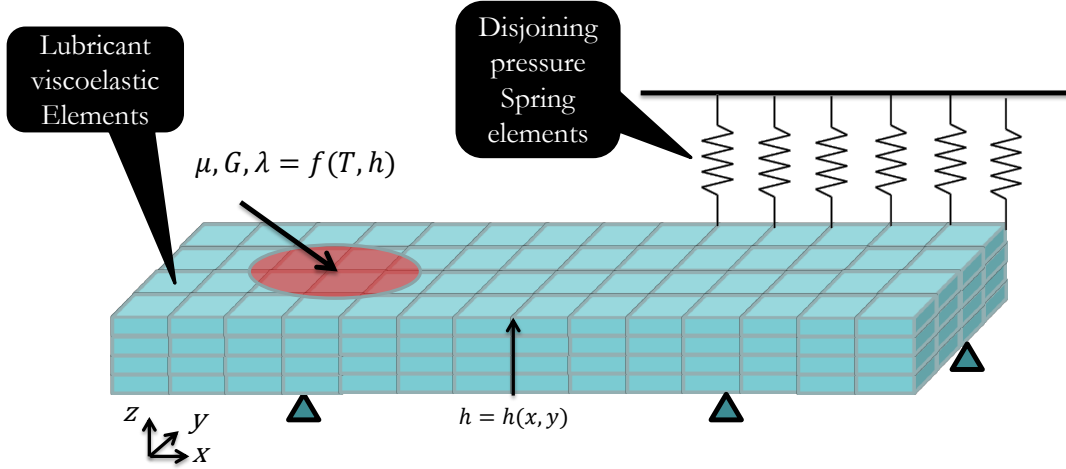
Figure 10.1: A schematic depiction of the 3D mesh used for FEA analysis of the problem.
