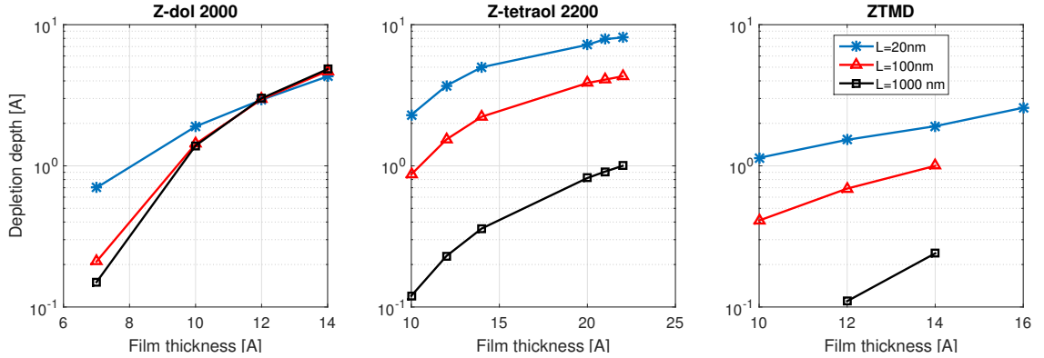
Figure 5.8: Trough depth as a function of the initial film thickness for different lubricant types, and different laser spot sizes of L = 20nm, 100nm, 1\mu m
