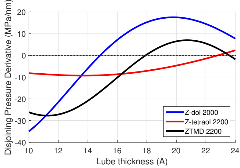
Figure 6.2: Disjoining pressure derivative d\Pi/dh as a function of lubricant thickness h for Z-dol2000 [15], Z-tetraol2200 [34], and ZTMD2200 [13].
