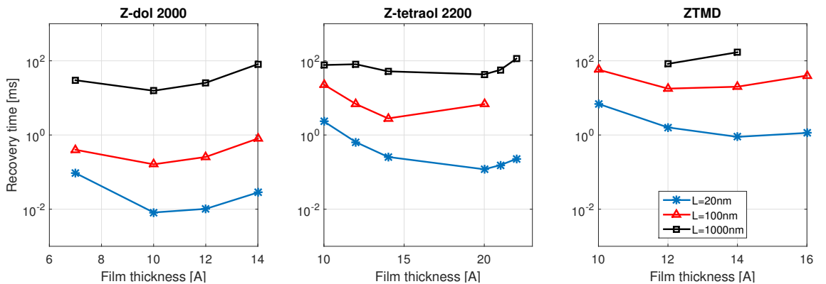
Figure 6.4: The recovery time as a function of the initial film thickness for different lubricant types, and different laser spot sizes of L = 20nm, 100nm, 1\mu m
