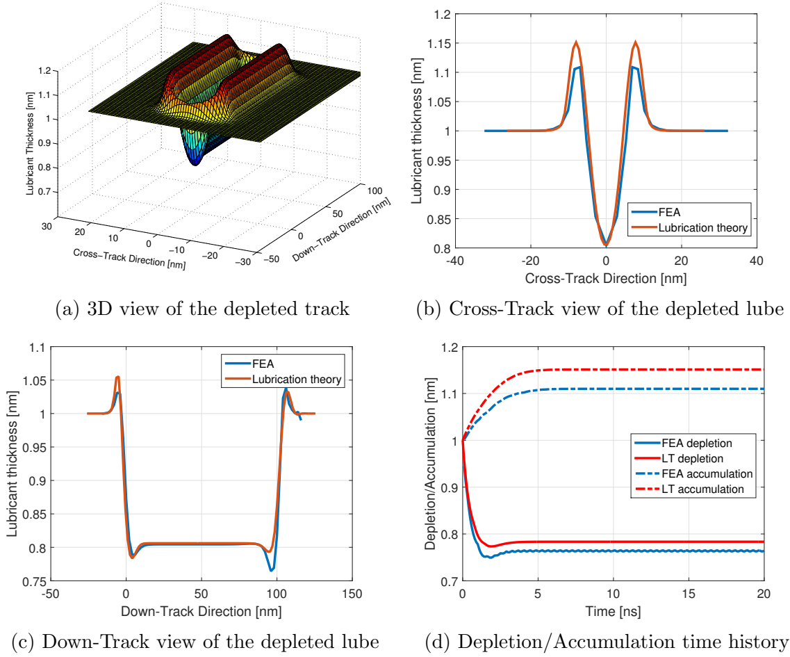
Figure 10.3: A comparison between results of viscous fluid using lubrication theory, and FEA with suppressed viscoelastic effects ( De = 0 )
