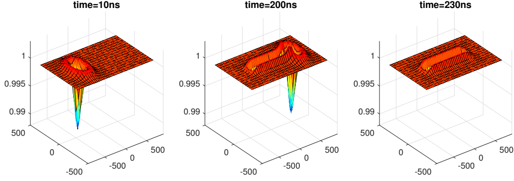
Figure 10.5: Viscoelastic FEA results for lubricant deformation and a laser spot size of L = 200nm a) right after the laser exposure, b) after a 200ns period, c) right after the laser exposure ends
