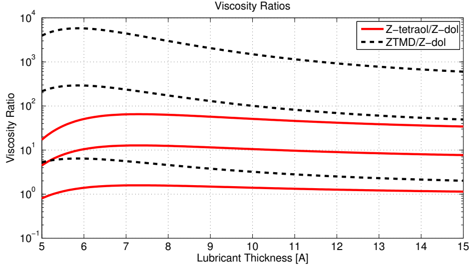
Figure 4.5: Thin-film effective viscosity ratio of Z-tetraol to Z-dol and ZTMD to Z-dol as a function of lubricant thickness for different temperatures for different lubricants. This is a comparison between these families of lubricants at temperatures T = \{20, 100, 300^\circ C\} . Higher curves correspond to lower temperatures (closer to room temperature)
