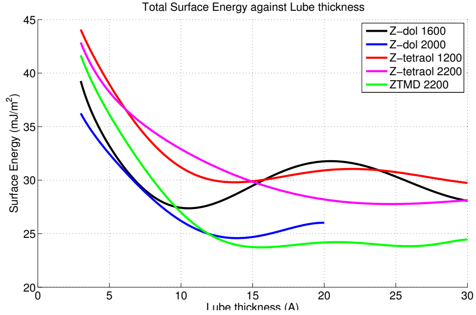
Figure 4.1: Total (sum of dispersive and polar components) surface energy as a function of lubricant thickness for Z-dol 1600, Z-dol 2000, Z-tetraol 1200, Z-tetraol 2200, and ZTMD. Surface Energy Parameters are calculated for both dispersive and polar components of the disjoining pressure for these lubricants according to Refs. [35], [32], [33], and [13]
