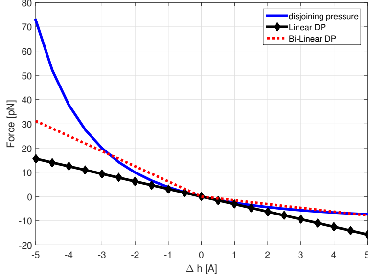
Figure 10.2: Nonlinear F(\Delta h) , linear F_L(\Delta h) , and bi-linear F_{BL}(\Delta h) Element Disjoining force as a function of lubricant thickness difference \Delta h
