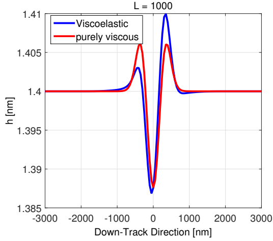
(a) Laser spot size L = 1\mu m
