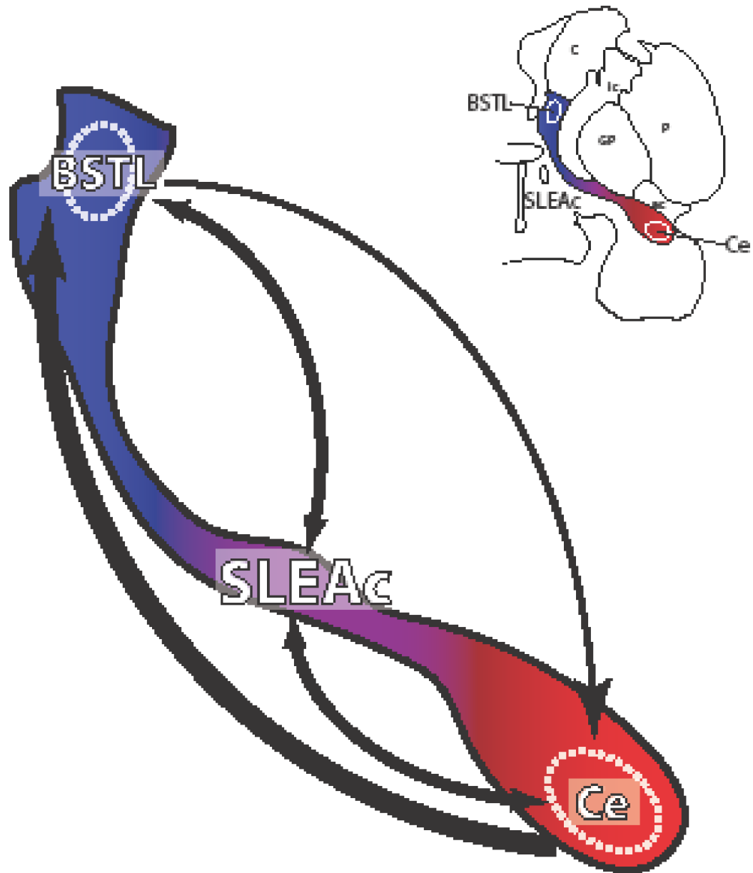
Figure 8. Overview of the intrinsic connections of the EAc. Direct long connections favor the Ce->BSTL direction over the BSTL->Ce path. However, the dense reciprocal innervation of the SLEAc, by both the BSTL and Ce, reveals a substrate for recurrent connections and underscores the SLE c's potential importance as a communication hub for extended amygdala information processing.
