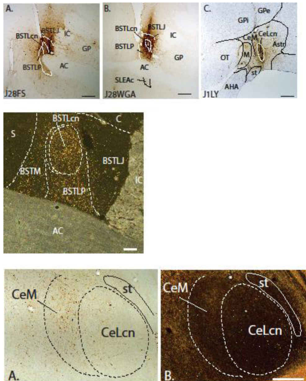
Figure 3. Row 1, A & B: Photomicrographs of representative injections into the BSTL (J28FS and J28WGA). Nuclear subdivisions were determined from adjacent sections stained for AChE. Case J28FS is centered on the BSTLJ and Case J28WGA is centered on the BSTLcn. C: A photomicrograph of an injection into the CeLcn (Case J1LY) with light cresyl violet counterstain. Note that the gliotic scar dorsal to injections site is due to DAB stain; there is no tracer uptake there. Scale bar = 1 mm. Row 2. Photomicrograph under dark-field illumination showing the distribution of labeled fibers in the BSTL subdivisions resulting from Case J9LY Scale bar = 500 \mu m. Row 3, A. A brightfield image of retrogradely labeled cells in the CeN subdivisions following an injection in the BSTL (Case J24FS). B. A
