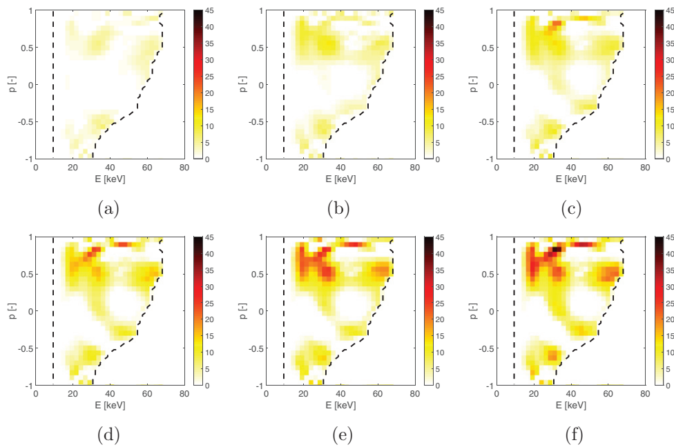
Figure 9. Inversions by TSVD with null-measurement constraint after NBI Q3 was turned on in discharge #33138 at t = 0.4 s. A movie is provided as supplementary material to this paper (movie 1) ( stacks.iop.org/NF/56/106024/mmedia ). NBI peaks at full, half, and one-third energy are gradually formed. The units are (10^{16} \text{ keV}^{-1} \text{ m}^{-3}) . (a) 0.40 s, (b) 0.42 s, (c) 0.44 s, (d) 0.47 s, (e) 0.49 s, (f) 0.52 s.
