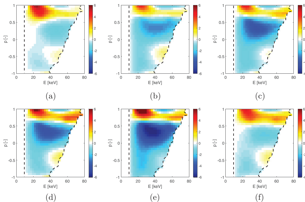
Figure 15. Reconstruction of the velocity-space distribution of the differences between the measurements and the TRANSP simulation \Delta F^* = F^* - F_{\text{sim}} ( 10^{16} \text{ keV}^{-1} \text{ m}^{-3} ) according to equation (10). Here the TRANSP simulations was used as prior information in the inversion. The crash occurs at t = 2.23 s. A movie is supplied as supplementary material to this paper (movie 3) ( stacks.iop.org/NF/56/106024/mmedia ). (a) 2.1 s. (b) 2.13 s. (c) 2.16 s. (d) 2.19 s. (e) 2.22 s. (f) 2.25 s.
