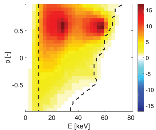
Figure 2. Comparison of the target velocity space identified in figure 1 with a TRANSP simulation of the fast-ion velocity distribution function ( 10^{16} \text{ keV}^{-1} \text{ m}^{-3} ). The simulation confirms the form of the null-measurement region with negligible phase-space densities. The colorbar is linear and includes positive phase-space densities as well as negative phase-space densities to allow comparisons with figures 4 and 5.
