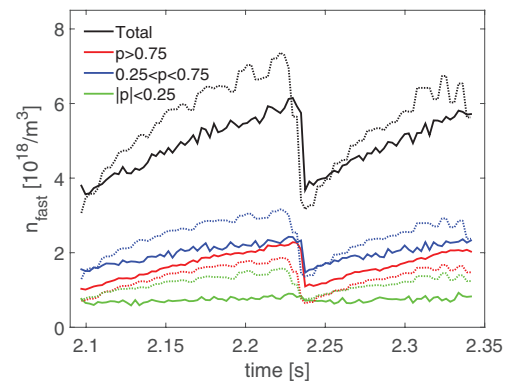
Figure 13. The measured (full lines) and simulated (dashed lines) total fast-ion densities and the fast-ion densities in selected pitch ranges in ASDEX Upgrade discharge #32323.
