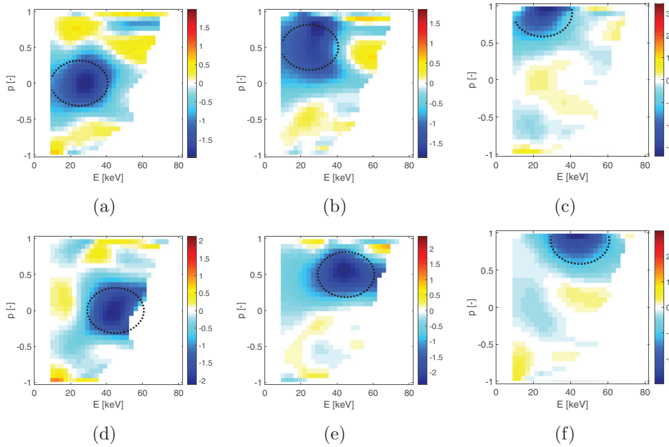
Figure 7. \Delta F^* = F^* - F_{\text{sim}} where F^* is calculated as in figure 6(d). In each subfigure the black dotted line shows the true location of the discrepancy. The units are (10^{16} \text{ keV}^{-1} \text{ m}^{-3}) . The colorbar is different for each plot.
