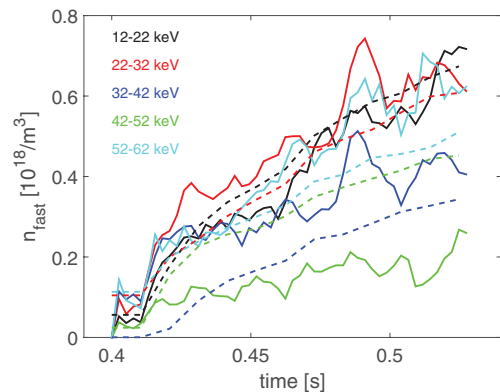
Figure 11. Measured (full lines) and simulated (dashed lines) increases in the fast-ion density for p \in [0.3, 0.7] and five 10 keV wide energy intervals in ASDEX Upgrade discharge #33138 right after the NBI is switched on. The fast-ion densities are obtained by integration of the high-definition tomographic inversion in the specified regions in velocity space. The fast-ion densities in the regions containing NBI peaks grow faster.
