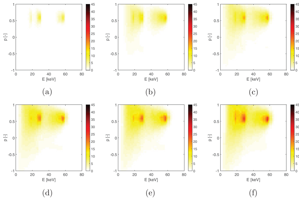
Figure 10. TRANSP simulation ( 10^{16} \text{ keV}^{-1} \text{ m}^{-3} ) as in figure 9 after NBI Q3 was turned on in discharge #33138 at t = 0.4 s. NBI peaks at full, half, and one-third energy appear in the simulation. (a) 0.40 s, (b) 0.42 s, (c) 0.44 s, (d) 0.47 s, (e) 0.49 s, (f) 0.52 s.
