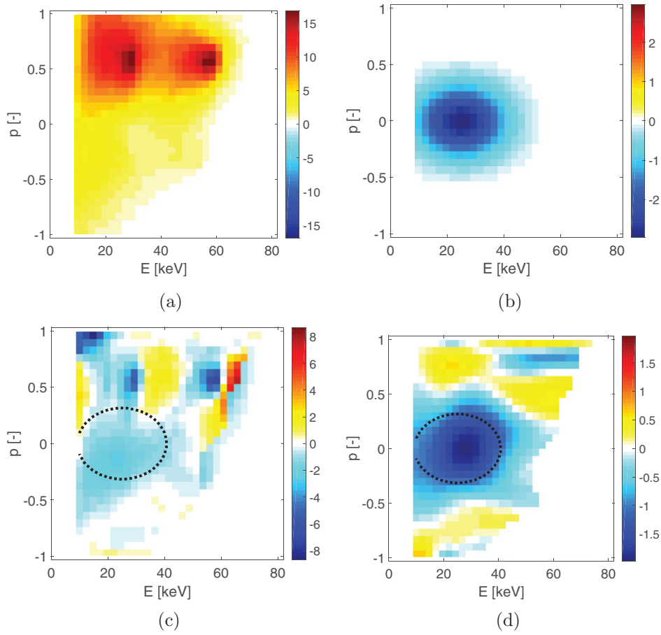
Figure 6. First-order Tikhonov tomographic inversions using a simulation as prior information. The units are (10^{16} \text{ keV}^{-1} \text{ m}^{-3}) . (a) F_{\text{true}} which is a modified TRANSP simulation with selective ejection of particles. (b) \Delta F = F_{\text{true}} - F_{\text{sim}} . (c) + (d) Inversion \Delta F^* = F^* - F_{\text{sim}} based on synthetic measurements of F_{\text{true}} with 5% Gaussian noise for a five-view FIDA system (c) without and (d) with the TRANSP simulation as prior information.
