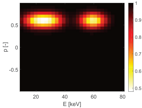
Figure 3. The known positions of the beam injection peaks are encoded by using a 2D regularization given by \kappa(E, p) [-]. The total regularization strength is given by \lambda\kappa(E, p) . The half- and one-third energy injection peaks merge due to the low resolution.
