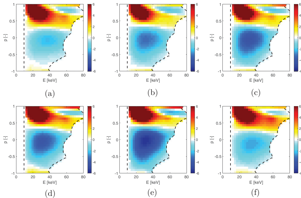
Figure 16. As for figure 15, but using only two FIDA views. The angles of the lines-of-sight to the magnetic field are \phi = [14^\circ, 73^\circ] . (a) 2.1 s. (b) 2.13 s. (c) 2.16 s. (d) 2.19 s. (e) 2.22 s. (f) 2.25 s.
