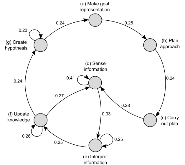
Figure 1: Sensemaking Processes from the Reverse Engineering Task
