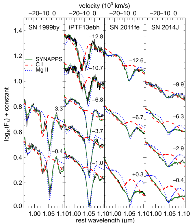
Fig. 8. The NIR C I \lambda 1.0693 \text{ }\mu\text{m} line for four SNe Ia with NIR C I detection. Each panel presents the time evolution for each supernova with the phase relative to B maximum labeled for each spectrum. The solid green curves are the best-fit SYNAPPS models. Dashed red and dotted blue curves show the isolated contributions from C I \lambda 1.0693 \text{ }\mu\text{m} and Mg II \lambda 1.0927 \text{ }\mu\text{m} , respectively. The velocity axes on the top are plotted with respect to the C I \lambda 1.0693 \text{ }\mu\text{m} line.
