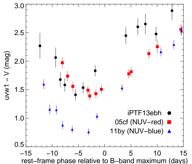
Fig. 6. The uvw1 – V color curves of iPTF13ebh, SNe 2005cf and 2011by. SNe 2005cf and 2011by are examples of the “NUV-red” and “NUV-blue” groups, respectively. The uvw1 – V color of iPTF13ebh is similar to that of the “NUV-red” group, but evolves faster.
