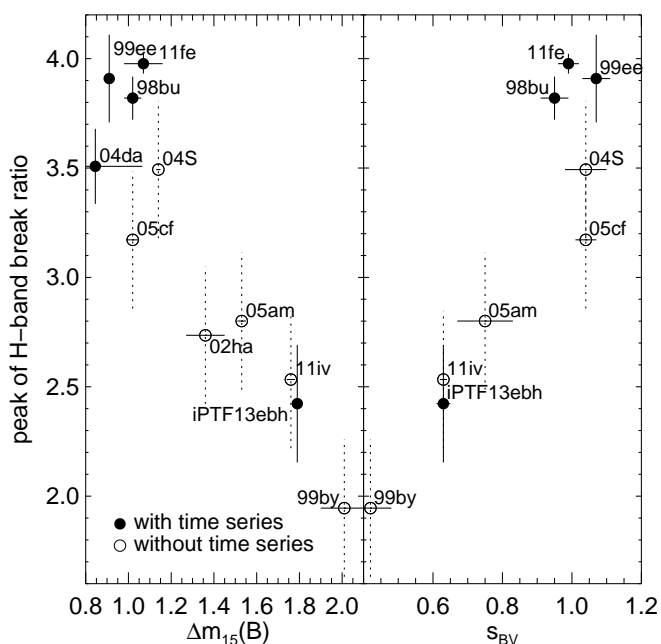
Fig. 14. The peak of H -band break ratio versus the optical light-curve decline rate \Delta m_{15}(B) and color stretch s_{BV} . SNe Ia with two or more observations in the post-peak decline are plotted with filled circles and solid error bars, while the rest are plotted with open circles and dotted error bars. The correlations for both parameters are strong.
