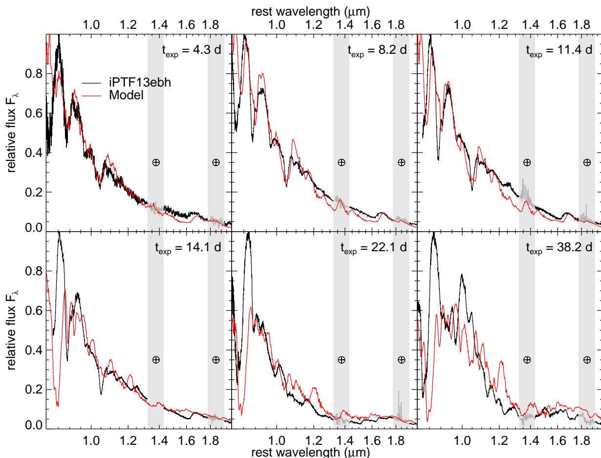
Fig. 12. Comparison between the NIR spectra of iPTF13ebh and the \rho_{tr} = 16 \times 10^6 \text{ g cm}^{-3} model spectra. The phases of the observed spectra are noted on the plot. These are relative to the explosion date, as inferred from the early-time r -band light curve. The model spectra are computed at these epochs.
