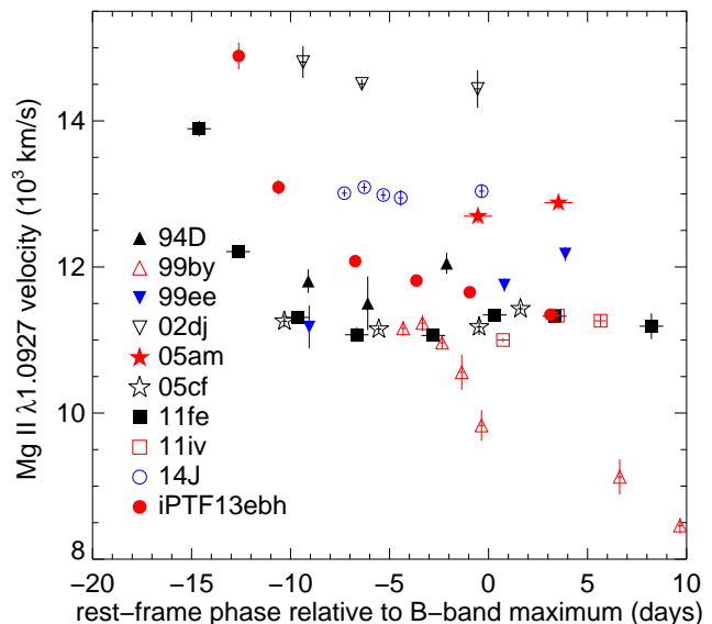
Fig. 16. The time evolution of the Mg II \lambda 1.0927 \mu\text{m} velocity. Various symbols represent different objects as noted on the plot. Blue, black, and red symbols represent SNe Ia with optical light-curve decline rates in the range \Delta m_{15}(B) < 1.0 , 1.0 < \Delta m_{15}(B) < 1.6 , \Delta m_{15}(B) > 1.6 , respectively. The Mg II \lambda 1.0927 \mu\text{m} velocity of iPTF13ebh decreases monotonically, indicating a deeper-reaching carbon burning layer than normal SNe Ia.
