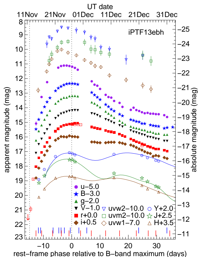
Fig. 2. UV, optical and NIR light curves of iPTF13ebh. The uvw2 , uvm2 and uvw1 light curves are obtained with UVOT on Swift; the uBVgri light curves are obtained with the e2v imager on Swope; and the YJH light curves are obtained with RetroCam on du Pont. All of these are without host subtractions. For the r -band light curve, open red square symbols represent host-subtracted r -band data from P48. A downward arrow marks the date of a non-detection image from P48 down to a magnitude limit of 21.7 mag. SNooPy fits (Burns et al. 2011) are plotted for the more sparsely-sampled NIR light curves. Blue and red vertical dash lines mark the dates when the optical and NIR spectra are taken, respectively. Two black vertical dotted lines are drawn at the inferred time of explosion and time of B -band maximum. The absolute magnitude is computed using a distance modulus of 33.63, derived from the host recession velocity of Woods et al. (2006)
