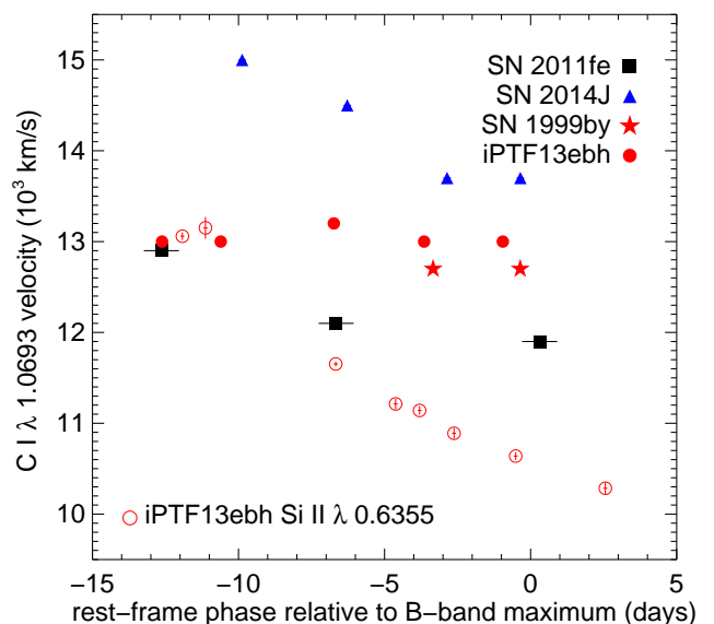
Fig. 9. The time evolution of the C I \lambda 1.0693 \mu\text{m} velocities for the four supernovae with C I detections. Various symbols represent different objects as noted. Blue, black, and red symbols represent SNe Ia with optical light-curve decline rates in the range \Delta m_{15}(B) < 1.0 , 1.0 < \Delta m_{15}(B) < 1.6 , \Delta m_{15}(B) > 1.6 , respectively. The velocities are taken from the C I velocity representing the base of the line-forming region in the best-fit SYNAPPS models. The Si II \lambda 0.6355 \mu\text{m} velocity of iPTF13ebh is also plotted for comparison.
