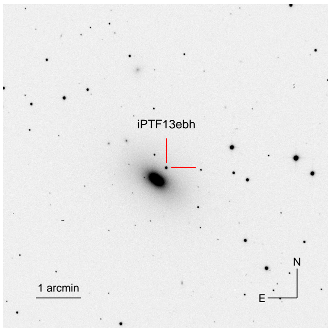
Fig. 1. A Swope r -band image of iPTF13ebh in NGC 890 taken near maximum light. The cross hair marks the location of the supernova. The compass and the size of the field are also noted.
