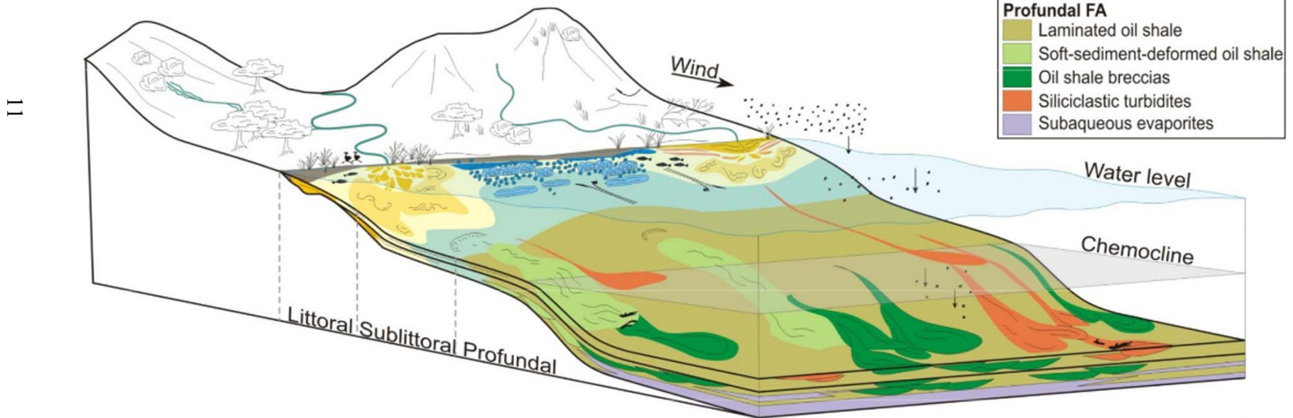
Figure 6. Depositional model for the Green River lake basins (modified from Tānavsū-Milkeviciene and Sarg, 2012)
