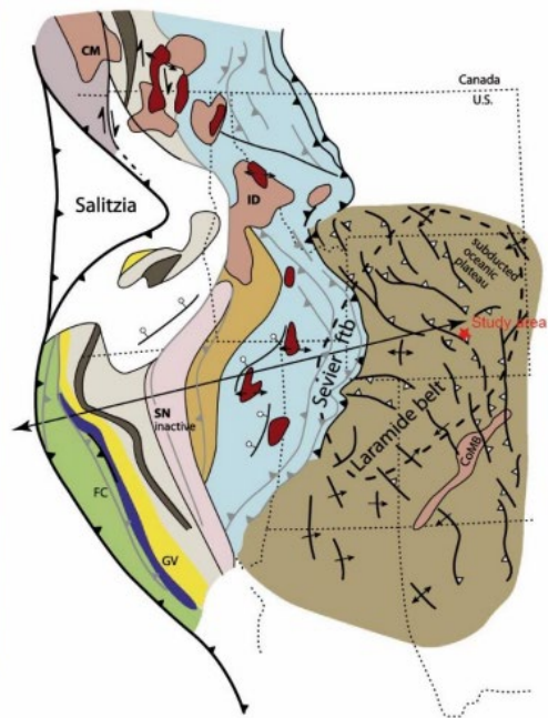
B - Structural map , Early Eocene ~50 Ma
