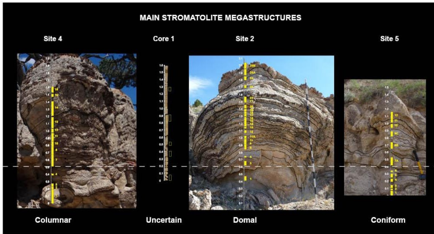
Figure 62. Main stromatolite megastructures sampled: columnar (site 4), uncertain (core 1), domical (site 2) and coniform (site 5). Samples are shown in yellow with respective identification number. Vertical scale (white numbers) in meters. Dashed white line is the correlation datum.
