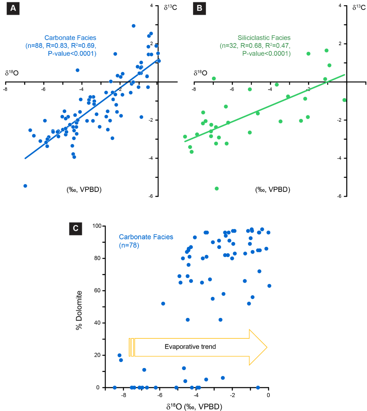
Figure 57. Stable isotope geochemistry: A) Carbonate facies: covariance of \delta^{13}\text{C} and \delta^{18}\text{O} data ( R>0.7 ) consistent with closed basin lake conditions (Talbot, 1990). Low p-value ( <0.05 ) means that the correlation is strong or important. (N = number of samples). B) Siliciclastic facies: \delta^{13}\text{C} versus \delta^{18}\text{O} plot with weak covariant trend ( R<0.7 ). C) Moderate-to-strong correlation between oxygen isotopic composition and dolomite content, indicative evaporative concentration (Arenas et al, 1997).
