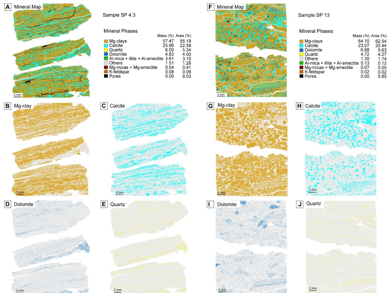
Figure 29. QEMSCAN Automated Mineralogical Mapping Results. Mg-claystone lithotype: A) Mineral spatial distribution with 10 \mu m resolution and quantification of mineral phases in area and mass; B to E) Mineralogical maps showing occurrence of Mg-clays, calcite, dolomite, and quartz. Mg-clay arenite lithotype: F) Mineral spatial distribution with a 10 \mu m resolution and quantification of mineral phases in area and mass; G to J) Mineralogical maps showing occurrence of Mg-clays, calcite, dolomite, and quartz.
