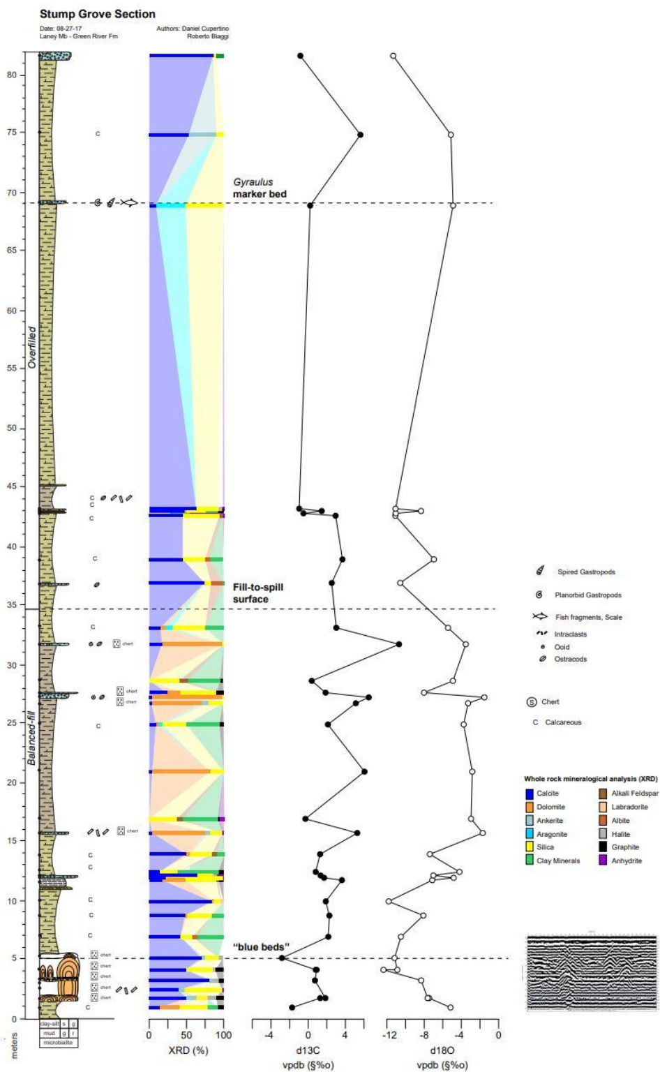
Figure 61. Stump Grove Section of Lower LaCledde Bed of the Green River Formation in the Vermillion Creek area. Note detailed lithology, XRD measurements, bulk rock (weight percent), and \delta^{13}\text{C} and \delta^{18}\text{O} stable isotopes.
