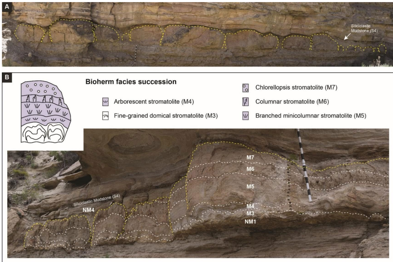
Figure 50. Bioherm facies succession: A) Individuals bioherms, west of Rosewood Section, showing distinctive domical shape (ranging in size from 0.4 to 1.5 m in height, and 0.5 to 5 m in diameter). B) distinctive facies succession within bioherms: fine-grained domical stromatolite facies (M3), followed by arborescent (M4) and branched minicolumnar stromatolites (M5), columnar stromatolites (M6), and Chlorellopsis (M7) facies at the top. Non-microbialite facies: Intraclastic conglomerate facies (NM1) and Ostracodal grainstone facies (NM4).
