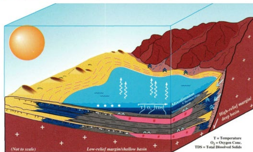
Figure 8. Schematic diagram highlights major features of overfilled, balanced-fill and underfilled lake basin types, which lake-level fluctuations are climatically driven (Bohacs et al., 2000).
