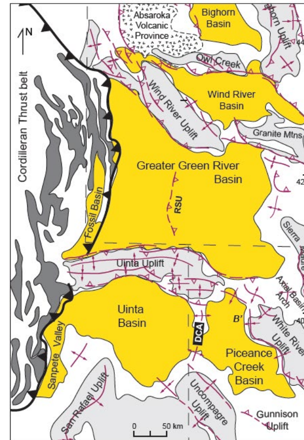
Figure 9. A) Two main Eocene lakes in which the Green River Formation was deposited: Lake Gosiute and Lake Uinta (modified from Blakey and Ranney, 2018). B) Cordilleran thrust belt (dark gray), intermontane basins (yellow) and basin-bounding uplifts (light gray) (modified from Dickinson et al. 1988, Smith and Carroll, 2015).
