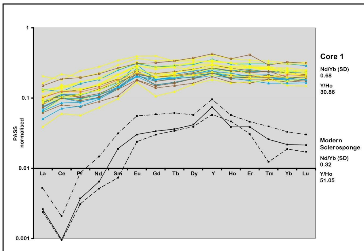
Figure 75. Rare earth elements and yttrium from different microbialite types in Core 1 (see figure 67 for color legend) and a modern marine sclerosponge (standard data supplied by Matthew Jackson).
