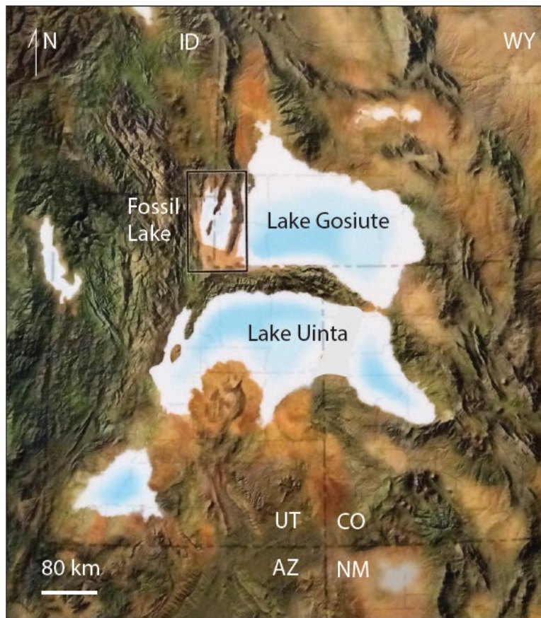
Figure 9. A) Two main Eocene lakes in which the Green River Formation was deposited: Lake Gosiute and Lake Uinta (modified from Blakey and Ranney, 2018). B) Cordilleran thrust belt (dark gray), intermontane basins (yellow) and basin-bounding uplifts (light gray) (modified from Dickinson et al. 1988, Smith and Carroll, 2015).
