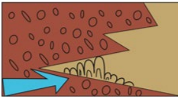
Figure 16. Stratigraphic occurrences of microbialites at transgressive phases of the Green River Formation (Buchheim, 2014).
