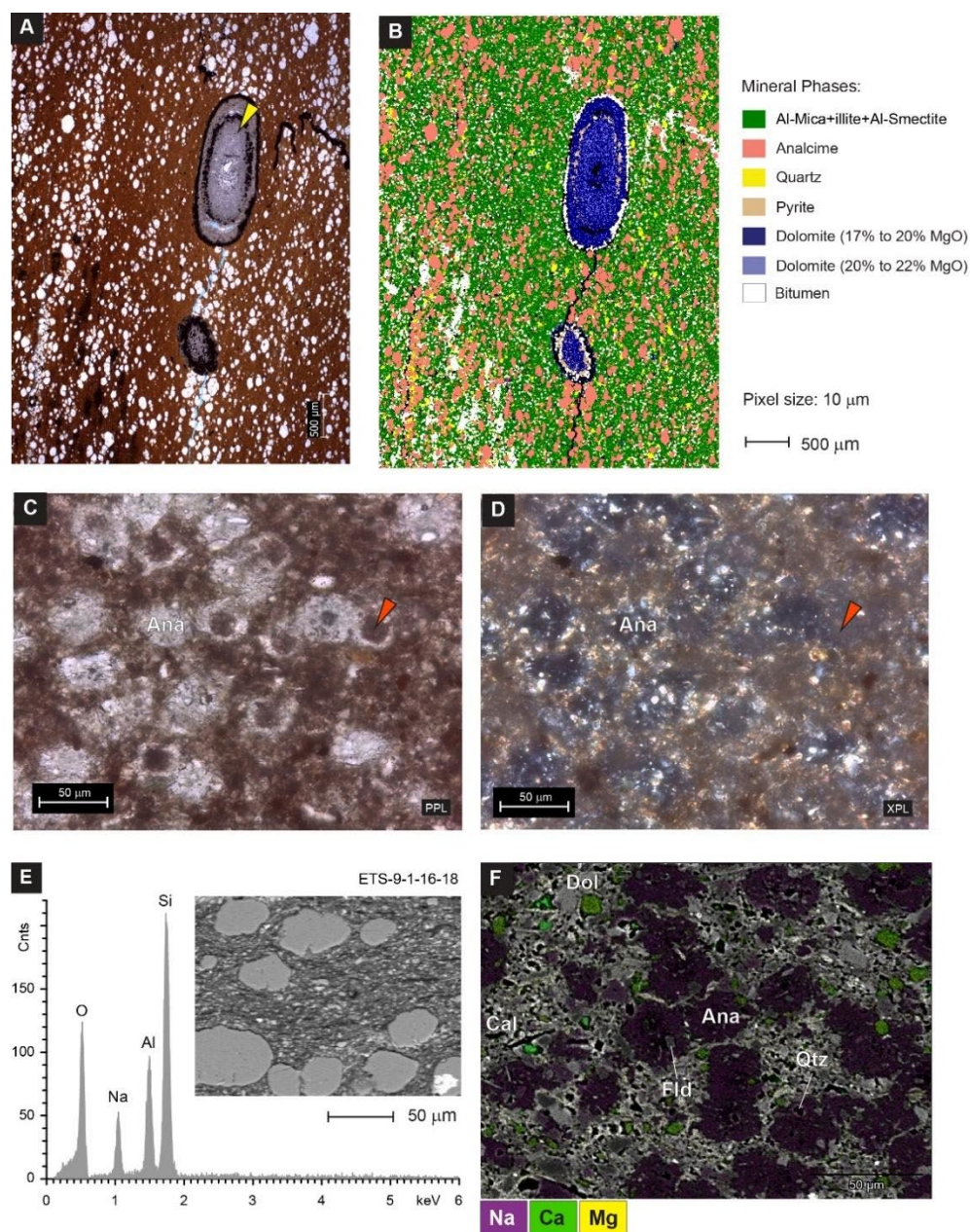
Figure 54. Analcime-rich siliciclastic mudstones: A) Thin-section photomicrograph showing amount and size of discrete analcime grains (10 to 80 \mu\text{m} ), ostracods (yellow arrow) and fine-grained minerals. Alizarine-red stained. B) QEMSCAN image of Fig. 54A, showing analcime minerals in a detrital clay matrix. Note ostracods grains replaced by Ca-dolomite. C) Thin-section photomicrograph of analcime-rich siliciclastic mudstones, showing subhedral analcime grains (Ana). Note authigenic analcime replacing the detrital clay mineral matrix (red arrow). D) Analcime minerals of Fig. 54C with isotropic extinction under crossed-polarized light (XPL). E) EDS spectrum typical for analcime grains present in siliciclastic mudstone facies (S3, S4). BSC-SEM Close-up of subhedral analcime granular crystals, note smooth surfaces; crystals are under 80 \mu\text{m} . F) BSC-SEM image and elemental maps from Fig. 54C. EDS Na element map (purple) showing grains fully composed by analcime mineral phase. EDS Ca element map (green) and EDS Mg element map (yellow) show occurrence of calcite (Cal) and dolomite (Dol) crystals.
