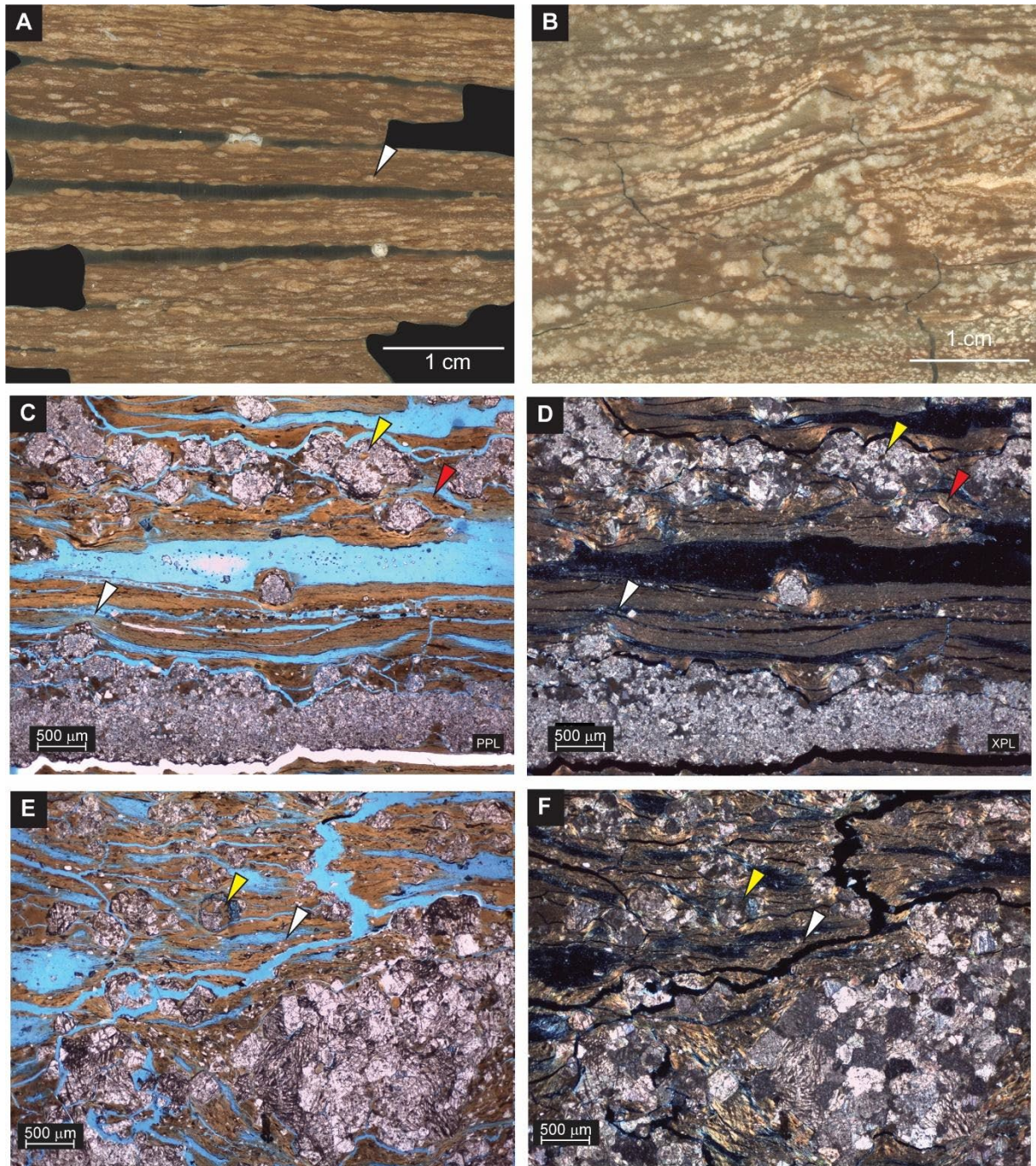
Figure 23. Mg-Claystone with Calcite Nodules. A) Laminated kerolite-stevensite claystone with calcite nodules (white arrow); B) K-S claystone with teepee structure and displacive calcite nodules and crystals; C) Micrite aggregates (nodules) displacing and replacing Mg-clay laminae (yellow arrow), that are shrunken and partially dissolved (white arrow) K-S laminations, displacing K-S laminations, and aggregates (red arrow) (PL); D) XPL; E) Calcite rhombs within K-S lamina (white arrow), K-S minerals preserved in calcite aggregates (yellow arrow) (PL); F) XPL.
