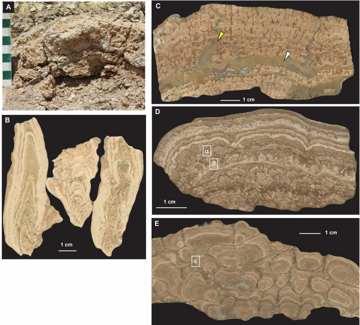
Figure 20. Types of Mg-clay stromatolites: A) Domical stromatolite (outcrop view); B) Columnar stromatolite; C) Minicolumnar stromatolites (mesostructure scale) with intercalated light (calcite) and dark (kerolite-stevensite mixed layered minerals (K-S)) laminae, early diagenetic silicification (white arrow) and late fracture-filling quartz (yellow arrow), slabbed sample of Fig.5A; D) Compound stromatolite (pseudocolumnar and minicolumnar stromatolites) with intercalated light (calcite) and dark (K-S) laminae. E) Nodular domical stromatolite.
