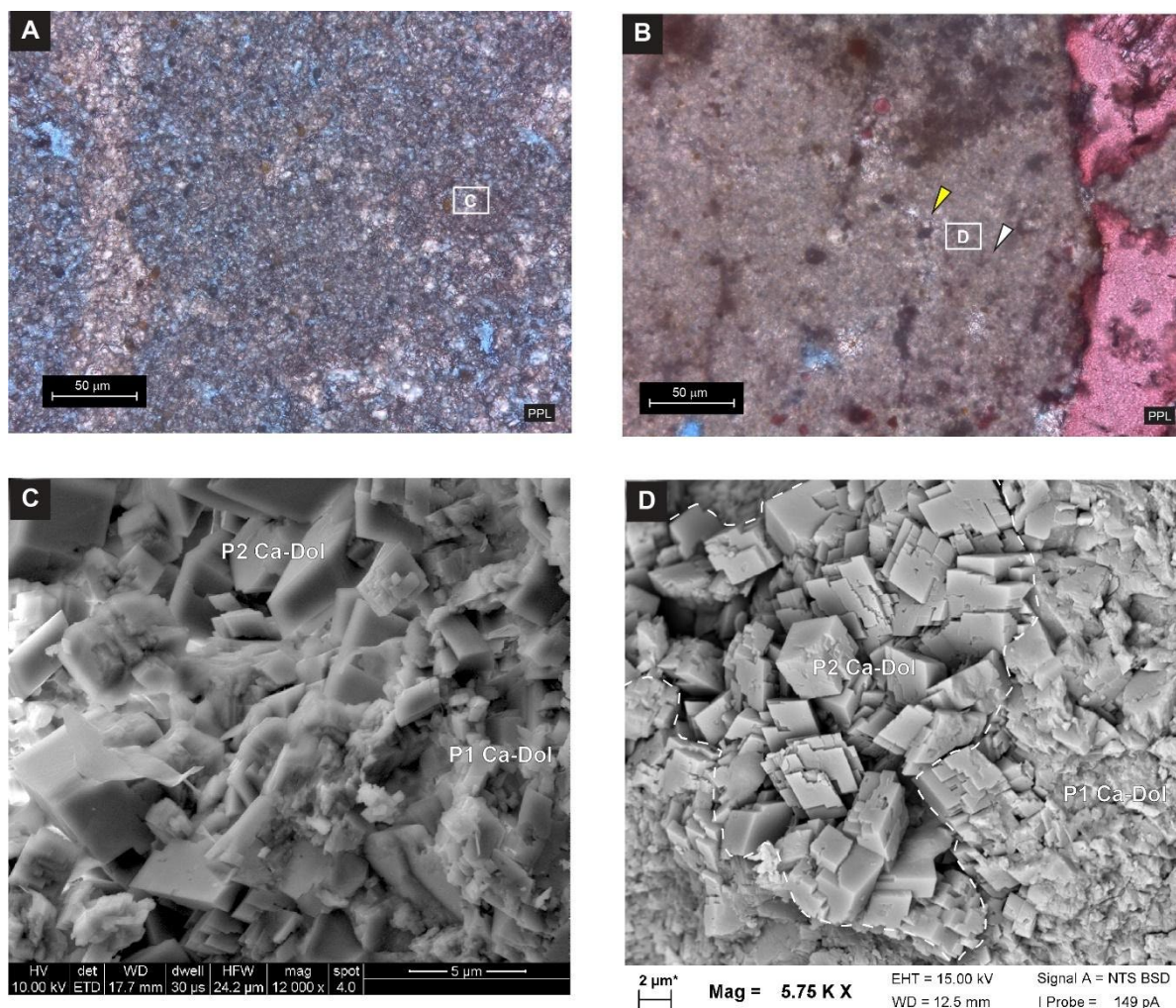
Figure 56. Two populations of Ca-dolomite microcrystals. A) Thin-section photomicrograph of Fine-grained domical stromatolite facies (M3, sample WSS-18) showing very fine dolomitic texture (mainly P2) with intraparticle porosity. B) Photomicrograph Branched minicolumnar stromatolite facies (M5, sample RS-Q5) showing a texture-preserving Ca-dolomite microrhombs (mainly P1): light brown zones (white arrow) composed of very fine dolomiticite (P1), whereas the dark brown are enclosed zones of organic matter; P2 crystals are present (yellow arrow). The void between the stromatolites here is filled by blocky calcite. C) SEM image of Fig.56A, note planar-e dolomite texture associated to P2 (>3 µm rhombs): flat dolomite faces and well-defined rhombohedral habit. D) SEM image of Fig.56B, planar-s dolomite texture associated to P1, very small Ca-dolomite rhombs (<3 µm) amidst in the anhedral to subhedral clusters of Ca-dol microcrystals and nanocrystals (<1 µm). Texture-preserving P1 Ca-dolomite microrhombs.
