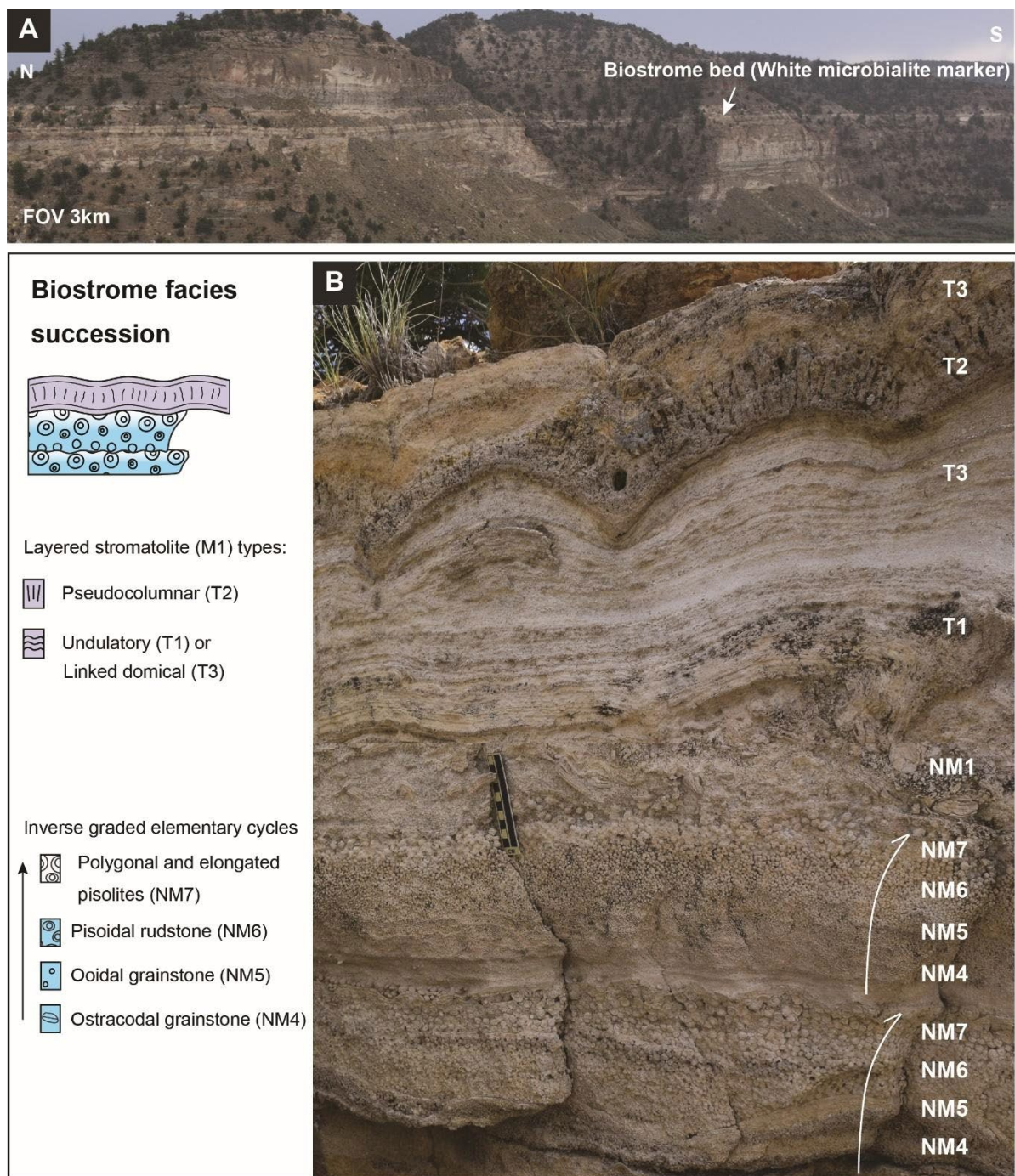
Figure 49. Biostrome facies succession: A) White microbialite marker bed, a tabular biostrome up to meter thick and traceable for kilometers. Photo taken south of Rosewood Section at Evacuation Creek. B) Outcrop view of well-developed inverse graded cycles.
