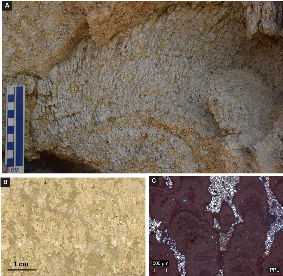
Figure 43. Branched minicolumnar stromatolite facies (M5): A) Outcrop view of branched minicolumnar stromatolites. Note some columns started out normal to the substrate and then bend to the right, which is southeast. B) Vertical slab of branched minicolumnar stromatolite. At the macrostructure level, columns are more slenderer and branch more frequently than stromatolites in M4. Laminae are not very evident. C) In thin section, laminae are evident with well defined, thin dark laminae and much thicker lighter laminae. Some laminae are discontinuous. Microstructure composed of dolomicritic. Note interspace infilled by fine-grained sediments that are coarser than those found in M4 (see Fig.55B for mineral composition).
