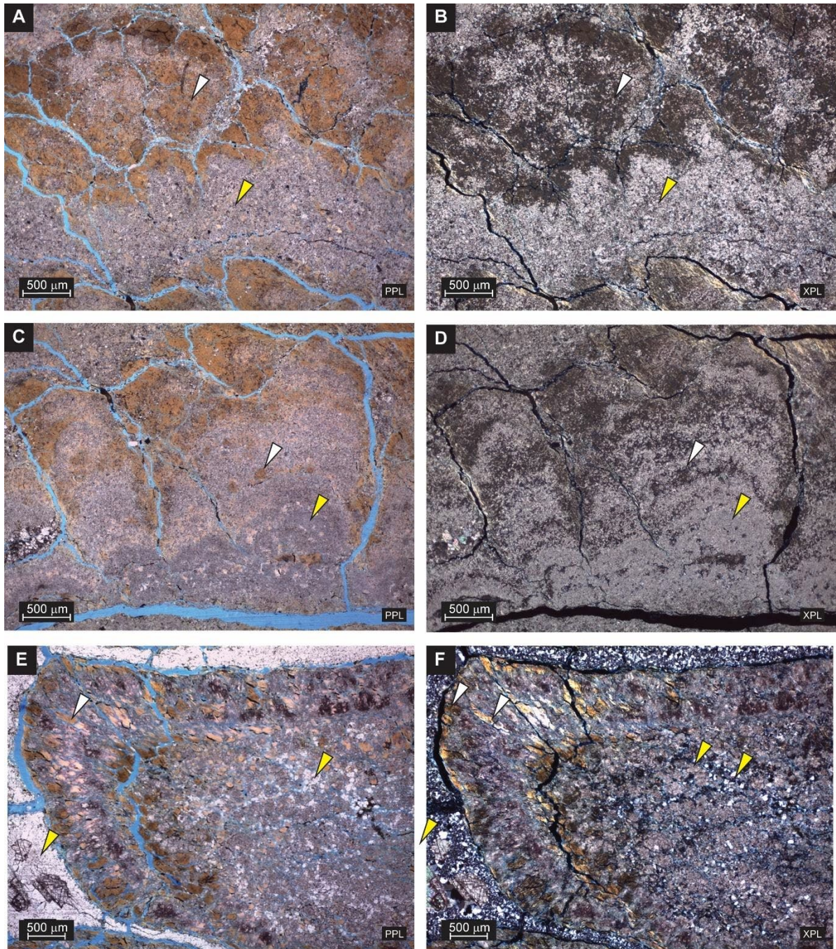
Figure 21. A) Minicolumnar stromatolite microstructure from Fig.4D(α). K-S crystal aggregates (white arrow), partially replaced by microcrystalline calcite crust (yellow arrow); plane-polarized light (PL); B) crossed-polarized light (XPL). C) Minicolumnar stromatolite microstructure from Fig.4D(β). Variable thickness of the micritic laminae (yellow arrow) intercalated with K-S crystal aggregates; some of K-S are partially replaced and engulfed by calcite crystals (white arrow) (PL); D) (XPL). E) Nodular domical stromatolite microstructure from Fig.4E(ε). Divergent radial K-S minerals (white arrow), within stromatolite nodules; partial dissolution and replacement by quartz crystals (orange arrow) and quartz mosaic cementation among nodules (yellow arrow) (PL); F) (XPL).
