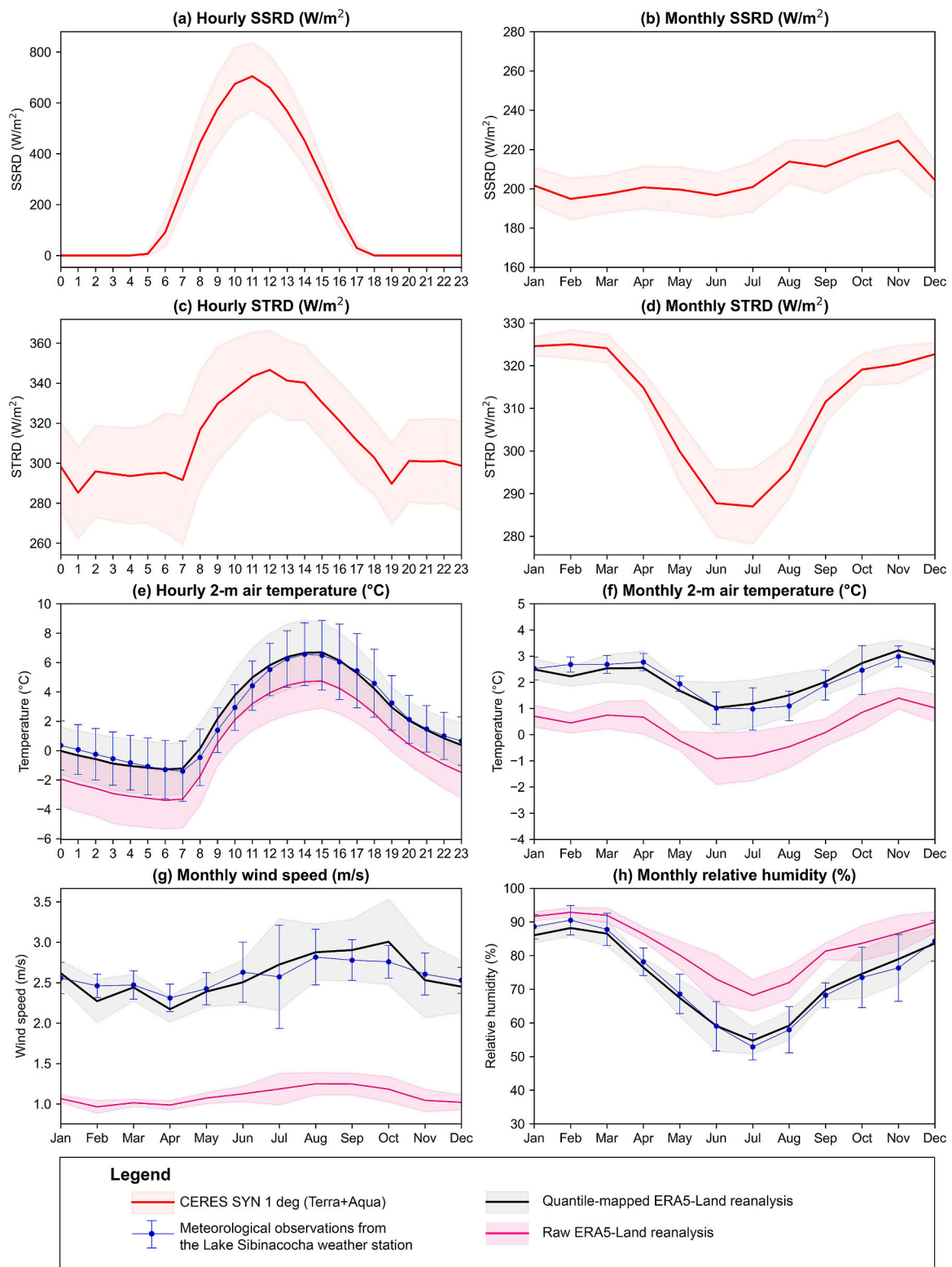
Fig. 2. Hourly and monthly climatologies of raw and quantile-mapped lake model input variables. (a) CERES surface shortwave radiation downwards hourly averages (SSRD; W/m^2 ). (b) CERES SSRD monthly averages ( W/m^2 ). (c) CERES surface thermal radiation downwards hourly averages (STRD; W/m^2 ). (d) CERES STRD monthly averages. The red lines and shadings in (a) – (d) are averages between March 2000 and December 2023 and their respective standard deviations. (e) 2-m air temperature (T2M) hourly averages. (f) T2M monthly averages. (g) wind speed monthly averages, and (h) relatively humidity monthly averages. The pink lines and pink shadings in (e) – (h) are averages and corresponding standard deviations from the raw ERA5-Land dataset (March 2016 – December 2023), while the black lines with gray shadings are the quantile-mapped ERA5-Land variables and their standard deviations. The blue lines with blue error bars are the mean and standard deviation of the observations from the Sibinacocha weather station. (For interpretation of the references to colour in this figure legend, the reader is referred to the web version of this article.)
