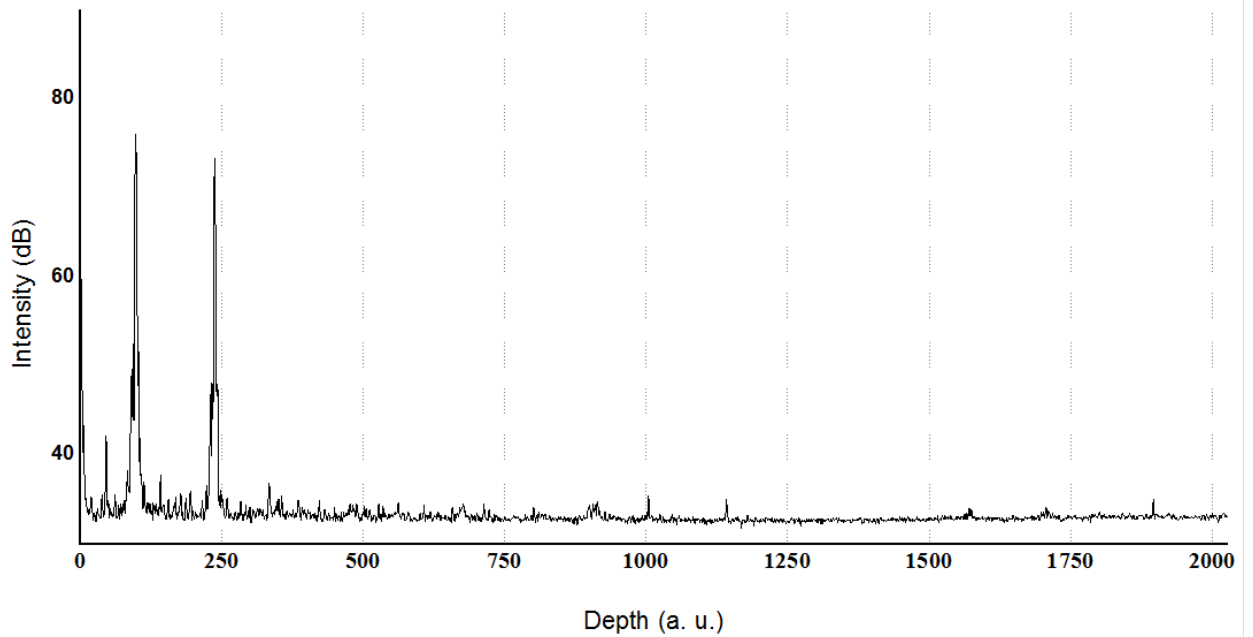
Fig. 3.6 Calibrated depth profile of a cover slip sample where two peaks, representing top and bottom layers of cover slip, are much better resolved than that in Fig. 3.1. The improved shows the effect of proper wavelength assignment.
