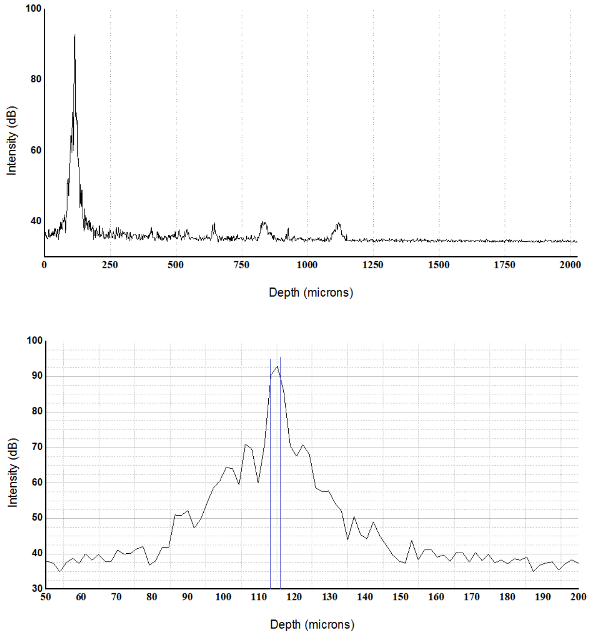
Fig. 3.7 Characterization of system axial resolution. (top) Depth profile of the sample when a mirror was placed as a sample. The distance from the zero position refers to the corresponding path difference between reference and sample arm. (bottom) The enlarged version of the peak shows how to calculate the axial resolution from the FWHM of the peak.
