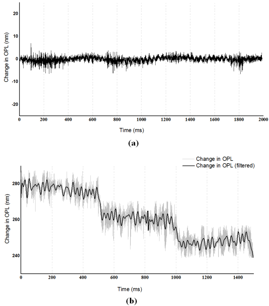
Fig. 4.6 Phase difference between two layers of cover slip measured over time. The standard deviation of this plot represents the phase noise margin or lower limit of detectable phase change (a). Pr-OCT detection of piezo-controlled 20nm stepwise displacements of a glass slide (b).
