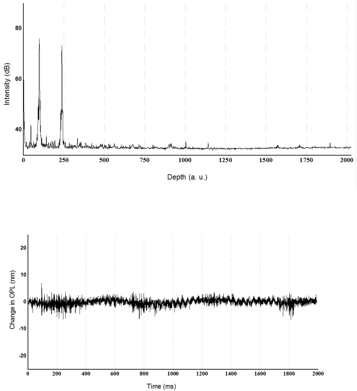
Fig. 3.15 Depth profile showing the cover slip peaks for its top and bottom layer (top). The change in phase difference between those two peaks over time. The standard deviation of these values represents the noise margin.
