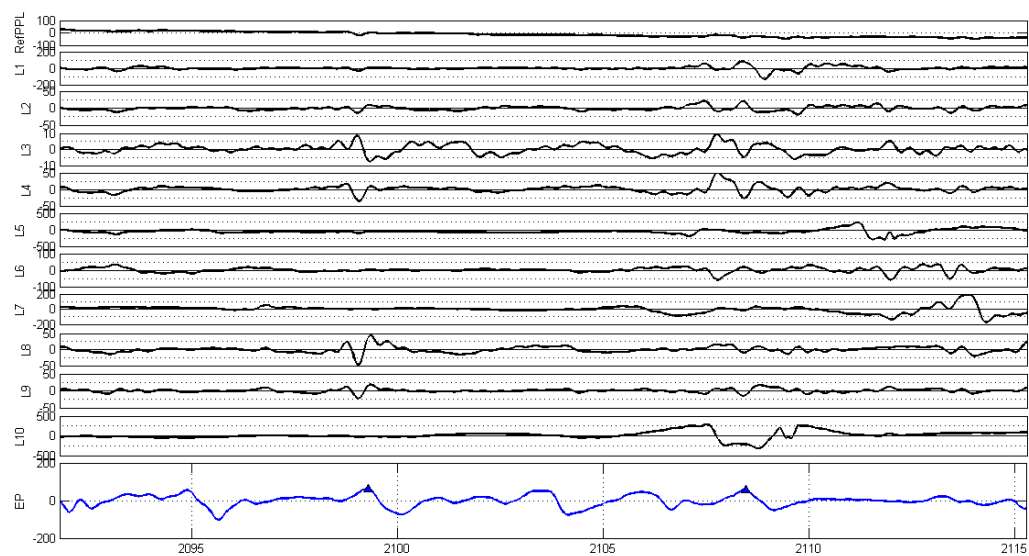
Fig. 4.16 Depth resolved activity (case 2)
